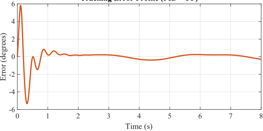
Tracking Error Profile (PID + FF)
