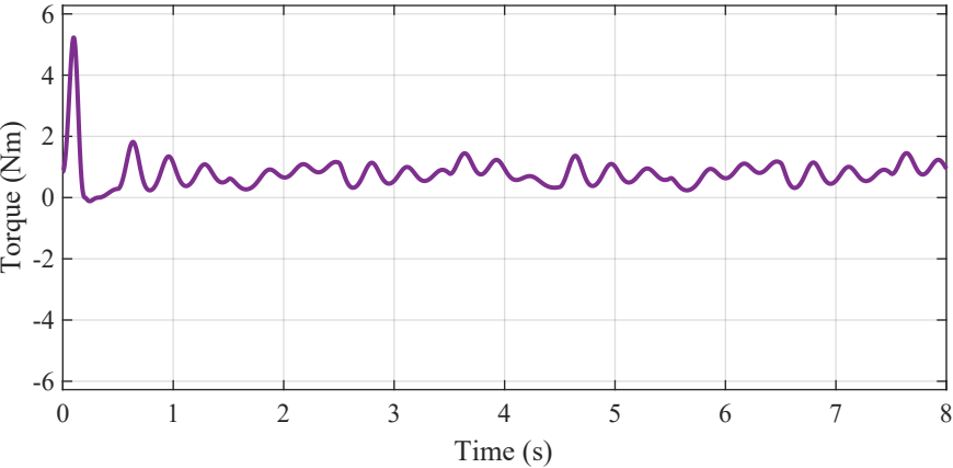
Propeller Generated Torque (PID + FF)
