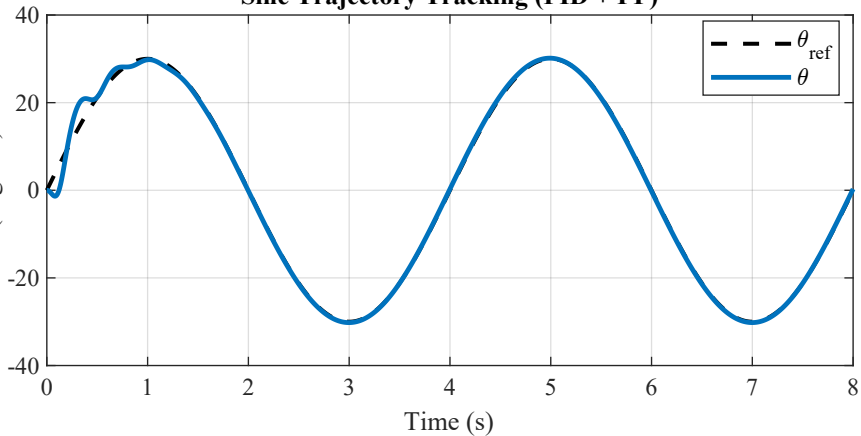
Sine Trajectory Tracking (PID + FF)
