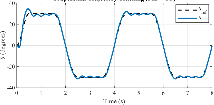
Trapezoidal Trajectory Tracking (PID + FF)
