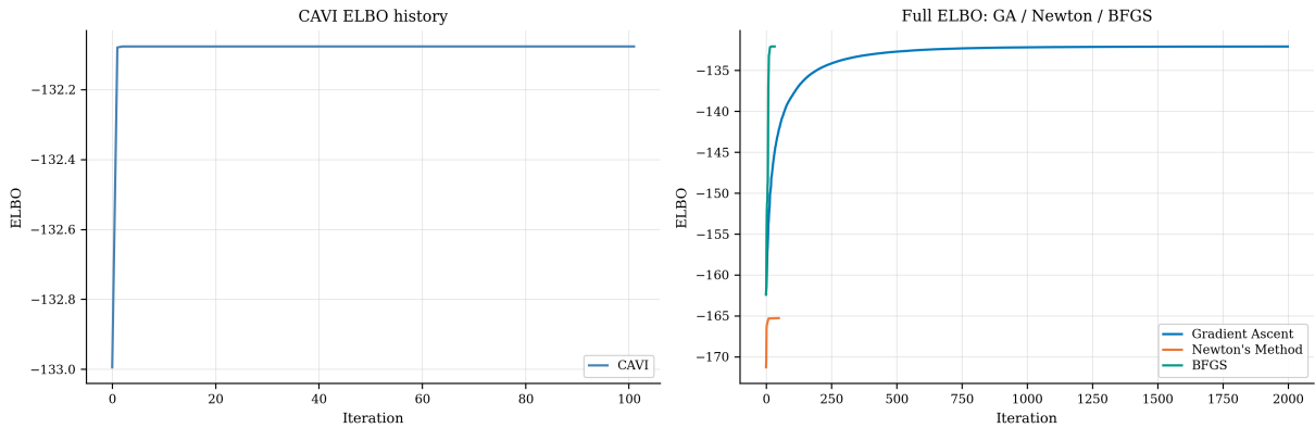
Figure 4: ELBO convergence for CAVI (left) and gradient-based methods (right). Newton's method converges to a suboptimal point; CAVI and BFGS agree.
