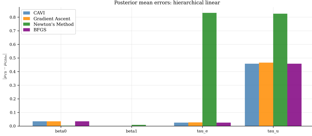
Figure 22: Absolute posterior mean errors relative to the Gibbs reference. Posterior means are accurate even where variance is collapsed.
