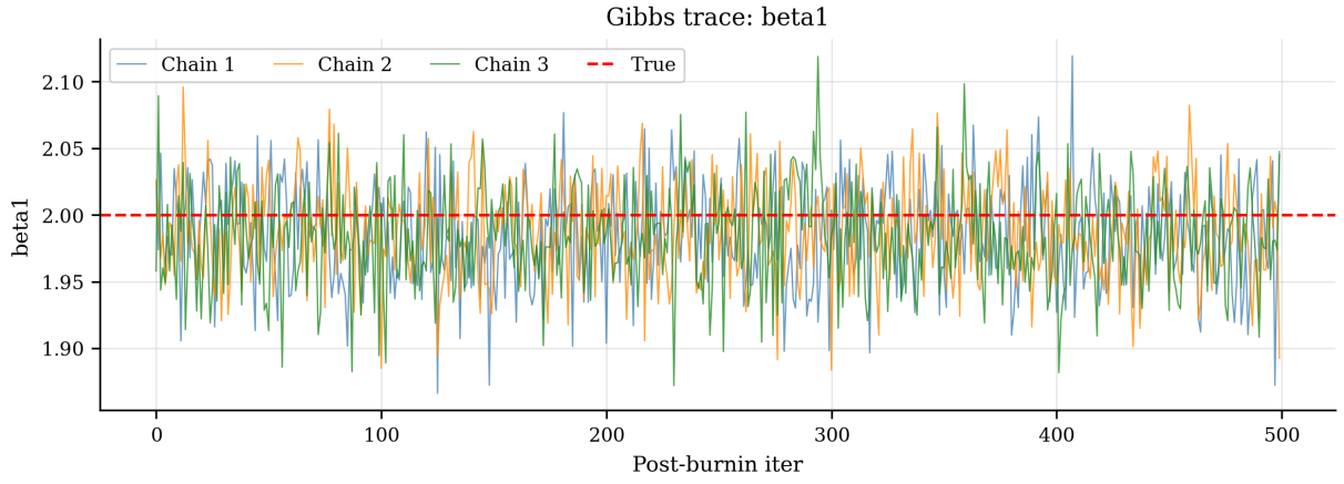
Figure 8: Gibbs trace: \beta_1 .
