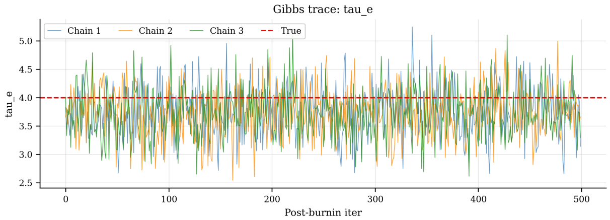
Figure 9: Gibbs trace: \tau_e (noise precision).
