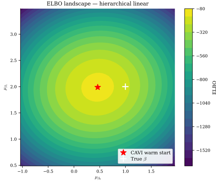
Figure 2: ELBO landscape slice in the (\mu_{\beta_0}, \mu_{\beta_1}) plane. Red star: CAVI warm start; white cross: true \beta .
