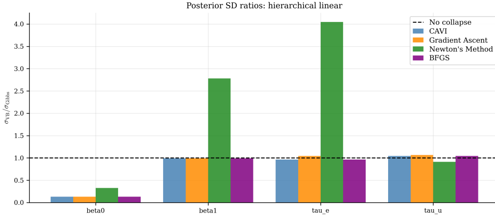
Figure 21: Posterior SD ratios (VI / Gibbs). Dashed line: ideal ratio 1.0. Severe intercept collapse ( \approx 0.13 ) for CAVI, gradient ascent, and BFGS.
