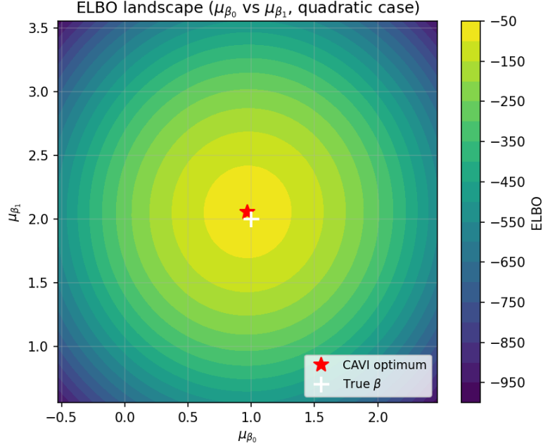
Figure 17: Two-dimensional ELBO slice for the quadratic case, varying \mu_{\beta_0} and \mu_{\beta_1} at the CAVI optimum. The star marks the CAVI solution.
