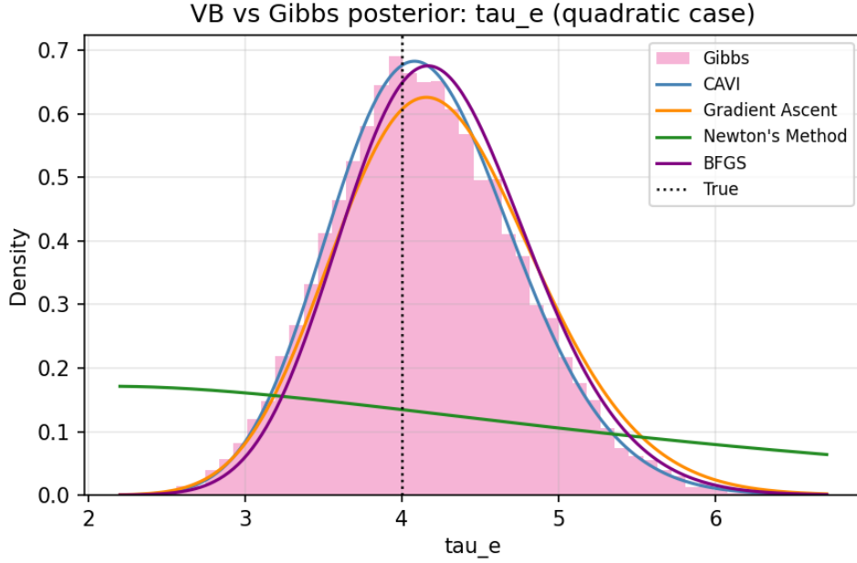
Figure 28: VB and Gibbs posterior densities for \tau_e (quadratic case). Newton's wide distribution reflects its over-dispersed critical point.
