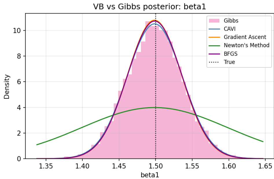
Figure 11: VB and Gibbs posterior densities for \beta_1 .
