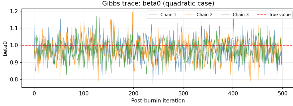
Figure 29: Gibbs trace plot for \beta_0 across 3 chains (quadratic case).
