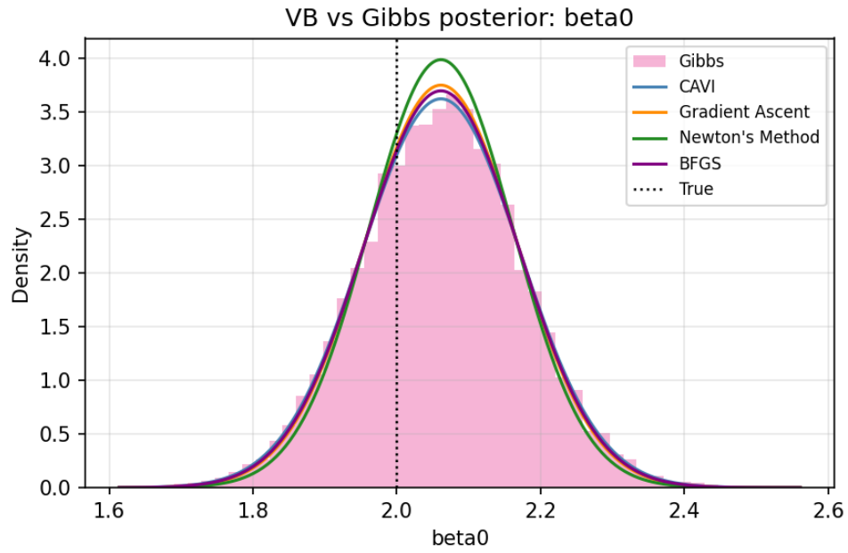
Figure 10: VB and Gibbs posterior densities for \beta_0 . The vertical dotted line is the true value.
