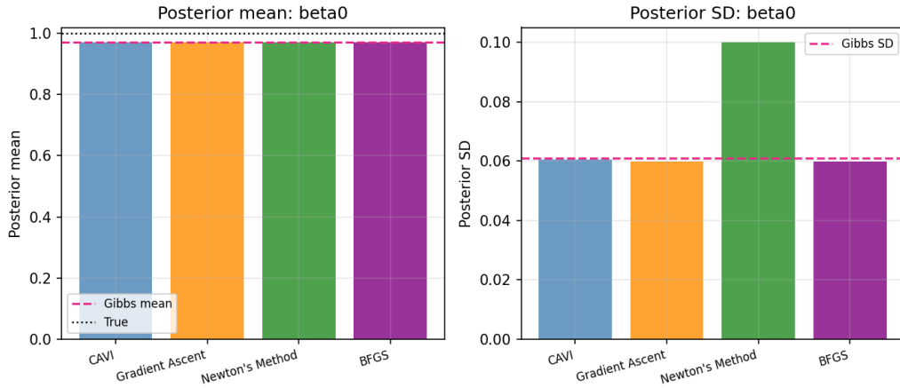
Figure 21: Posterior mean (left) and SD (right) for \beta_0 (quadratic case). Pink dashed: Gibbs. Black dotted: true value.
