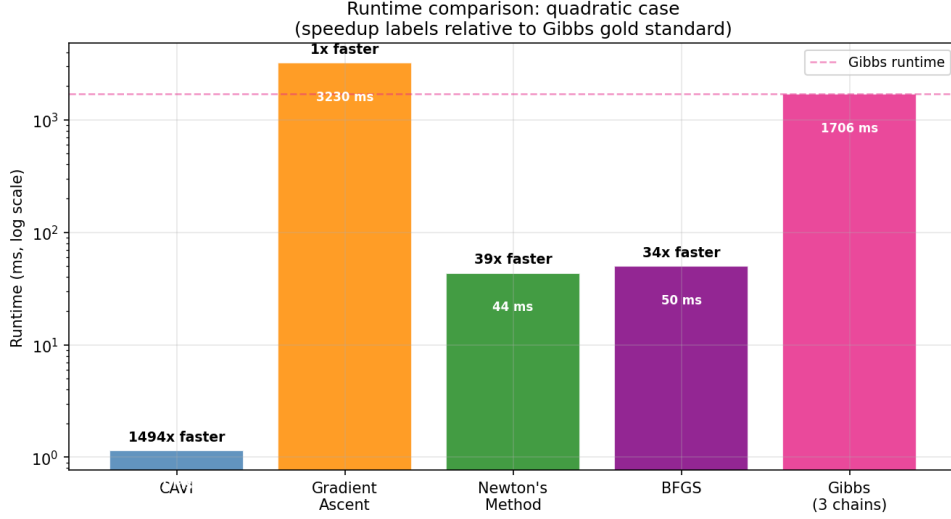
Figure 18: Computational cost on a log scale (quadratic case). Gradient Ascent is slower than Gibbs due to finite-difference overhead; CAVI remains the fastest method.
