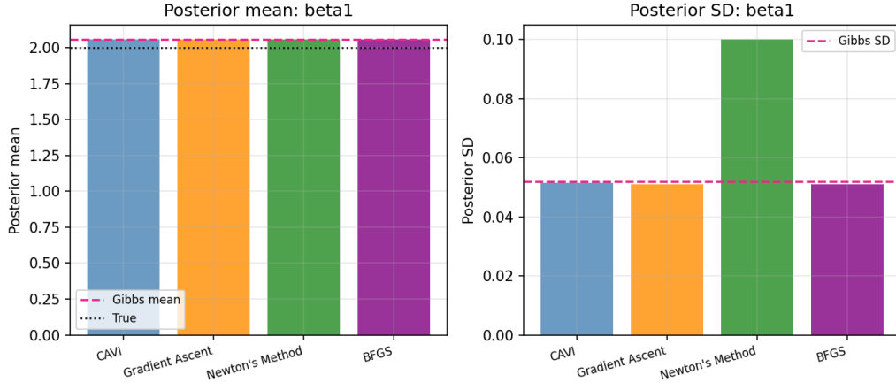
Figure 22: Posterior mean and SD for \beta_1 (quadratic case).
