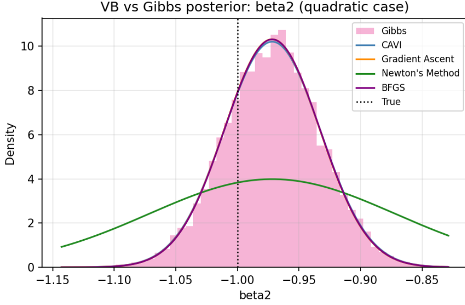
Figure 27: VB and Gibbs posterior densities for \beta_2 (quadratic case).
