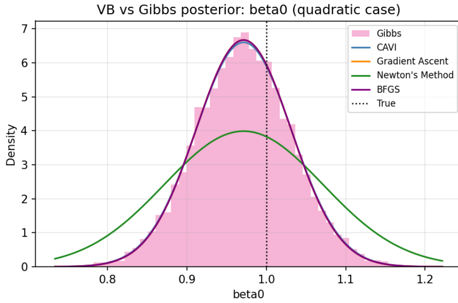
Figure 25: VB and Gibbs posterior densities for \beta_0 (quadratic case).
