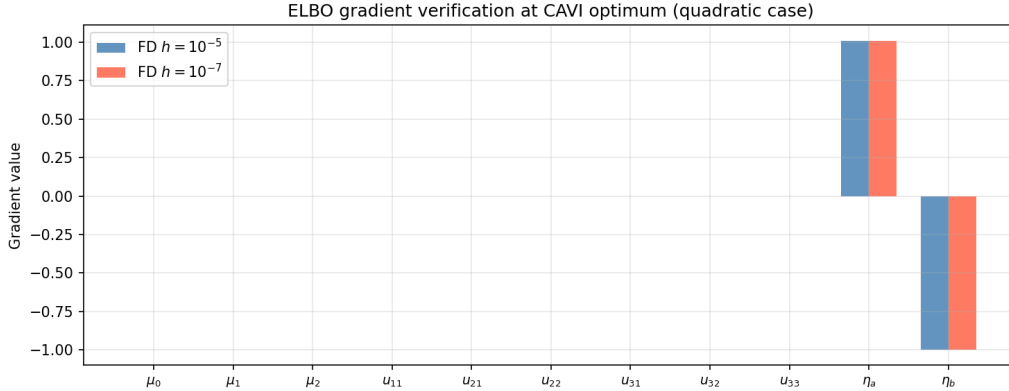
Figure 16: Gradient verification bar chart for the 11-parameter quadratic case. The two FD step sizes coincide visually for all components.
