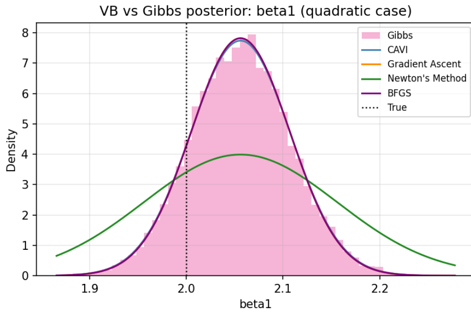
Figure 26: VB and Gibbs posterior densities for \beta_1 (quadratic case).
