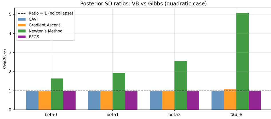
Figure 20: SD ratios \sigma_{\text{VB}}/\sigma_{\text{Gibbs}} for all four parameters (quadratic case). Newton's Method over-disperses dramatically for \beta_2 and \tau_e .
