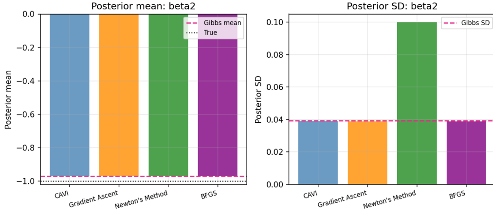
Figure 23: Posterior mean and SD for \beta_2 (quadratic case).
