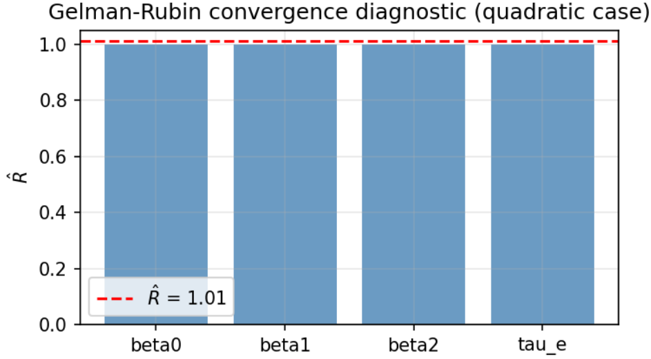
Figure 30: Gelman–Rubin \hat{R} for all four parameters (quadratic case). All values are below the convergence threshold of 1.01.
