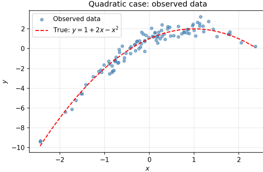
Figure 15: Generated quadratic regression data ( n = 100 ). The dashed curve is the true regression function \beta_0 + \beta_1 x + \beta_2 x^2 .
