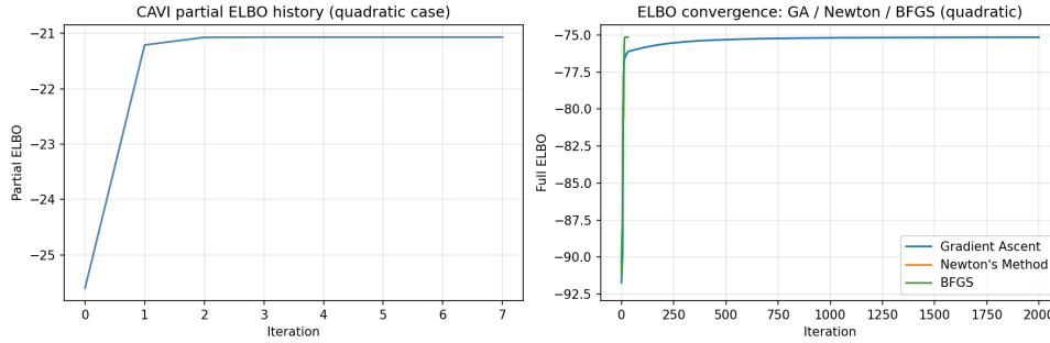
Figure 19: ELBO vs. iteration for the quadratic case. CAVI (left panel) converges monotonically; gradient-based methods (right) plateau well below the CAVI optimum.
