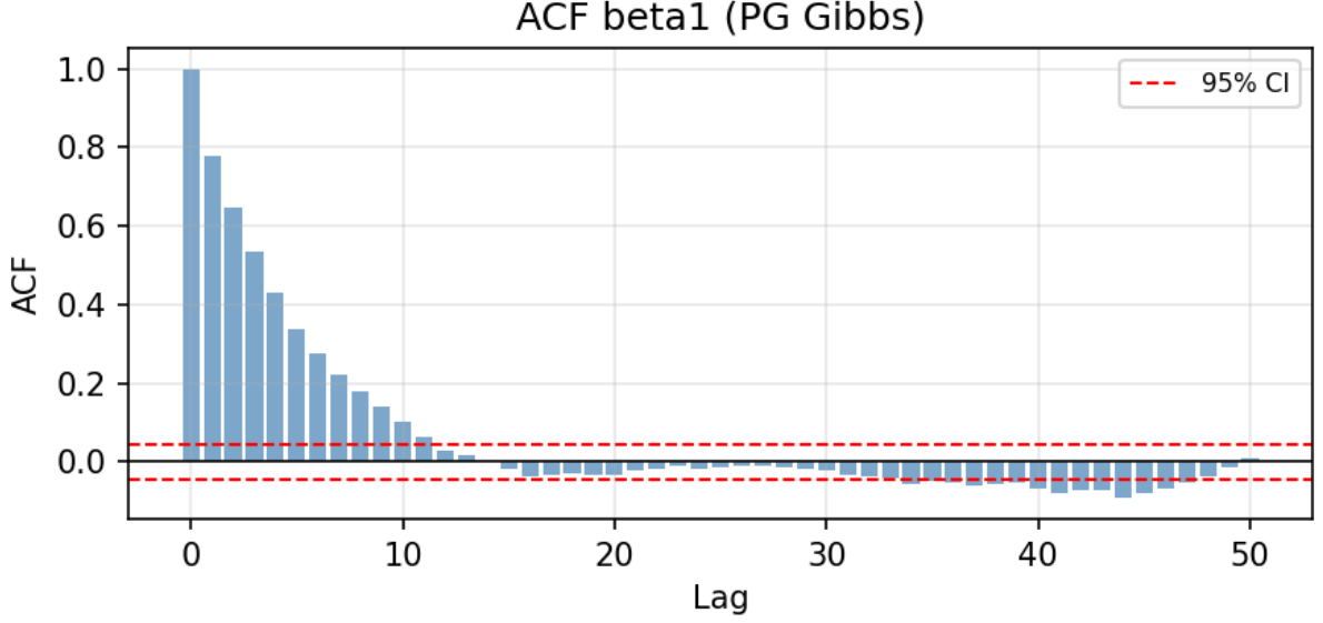
Figure 10: Autocorrelation function for \beta_1 .
