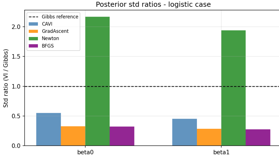
Figure 15: Posterior standard-deviation ratios (VI / Gibbs) for each method and parameter. The dashed line marks the ideal ratio of 1.0. Values below 1 indicate collapse.
