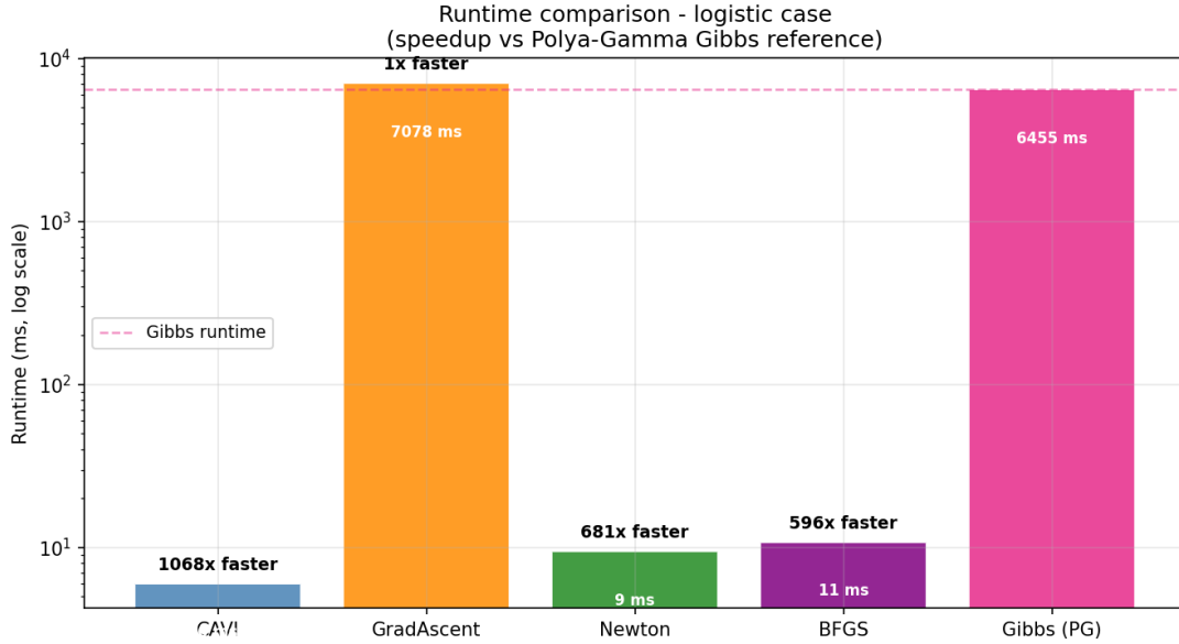
Figure 19: Computational cost on a log scale. Annotations give speedup relative to the PG Gibbs reference (dashed line). Note that cross-model timing comparisons (vs. the linear and quadratic cases) are qualitative only: the PG sampler requires n \times T = 10\,000 Gamma variates per iteration.
