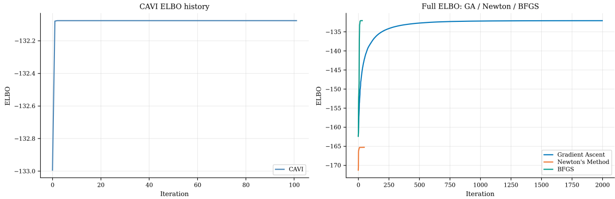
Figure 4: ELBO convergence for CAVI (left) and gradient-based methods (right). Newton’s method converges to a suboptimal point; CAVI and BFGS agree.
