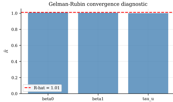
Figure 13: Gelman–Rubin \hat{R} diagnostic. All values below 1.01 confirm chain convergence.
