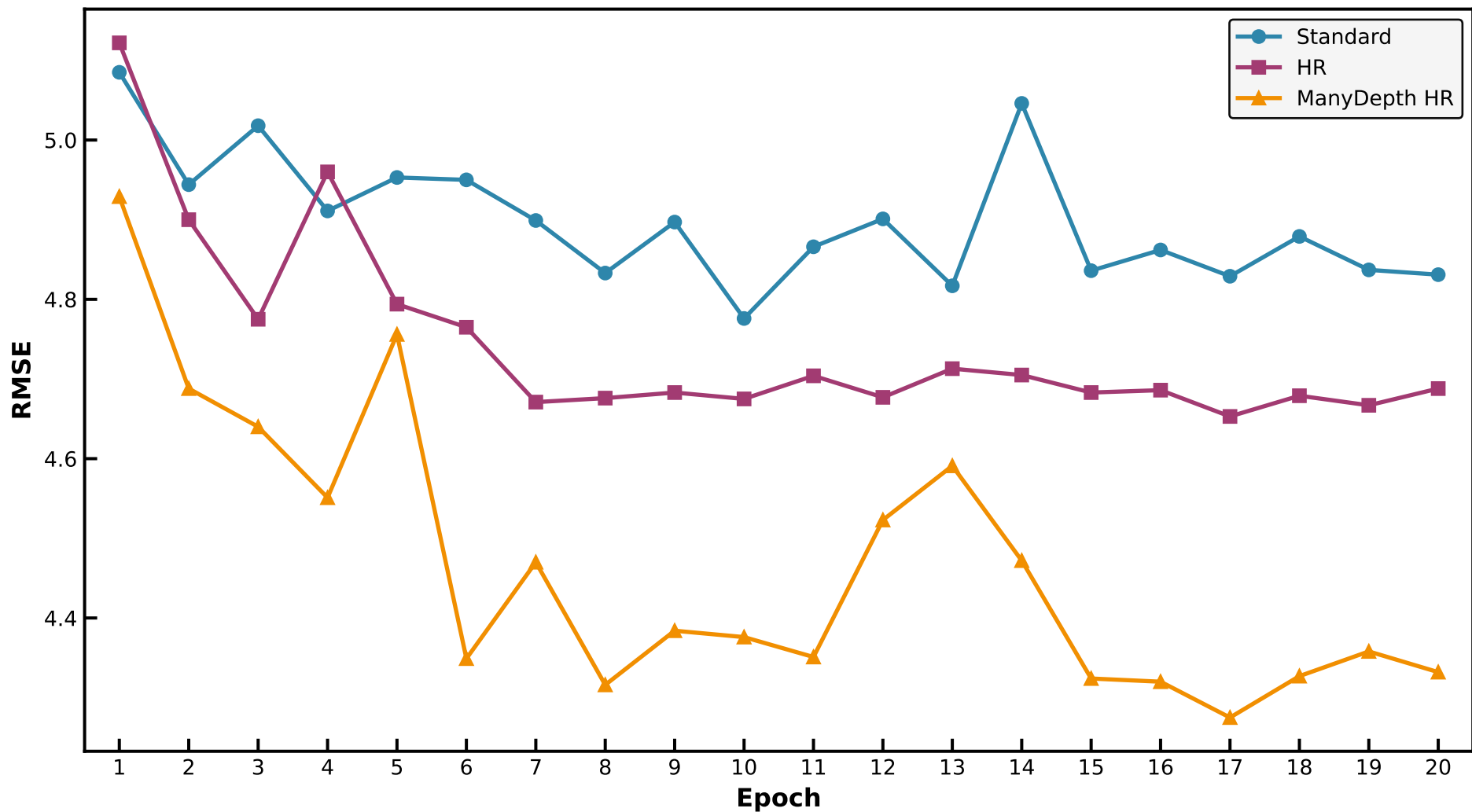
RMSE across Training Epochs
