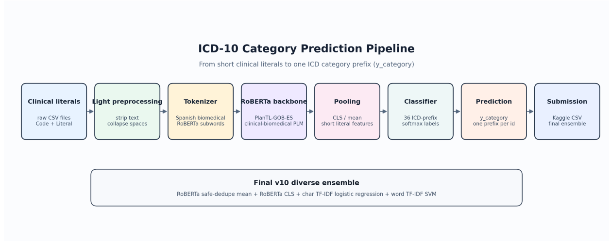
Figure 7: Final project architecture: data, light preprocessing, tokenizer, RoBERTa backbone, pooling/classification, prediction, and the final diverse ensemble used for submission.
