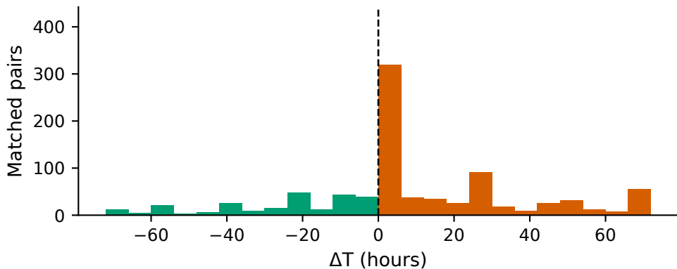
Personalised, 3 branches: N = 914, anticipation 26.6%
