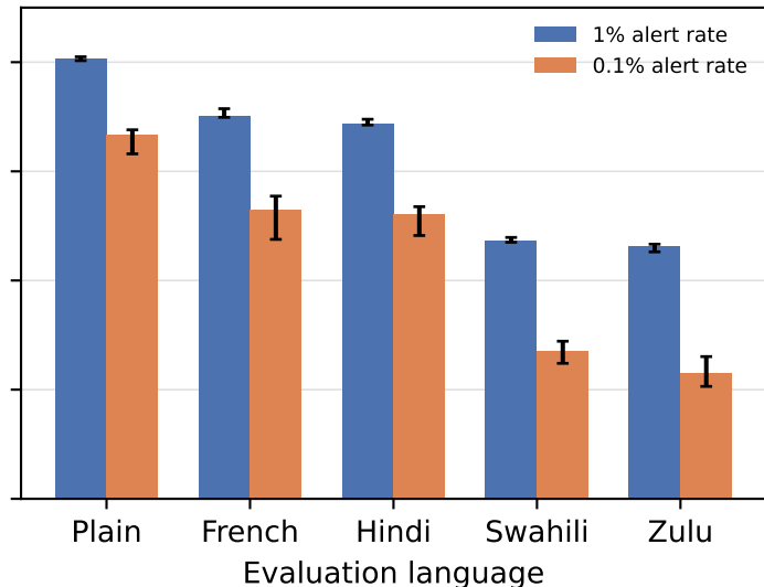
(b) WildChat threshold
