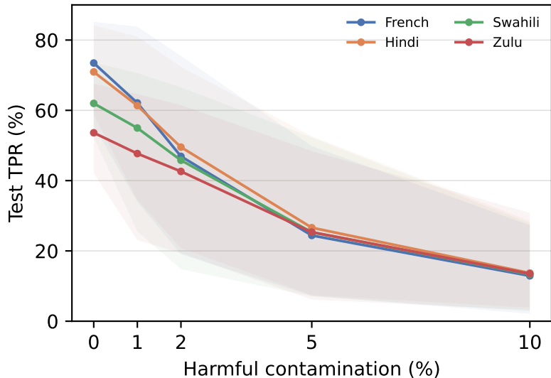
(a) Contamination sensitivity ( k = 300 )
