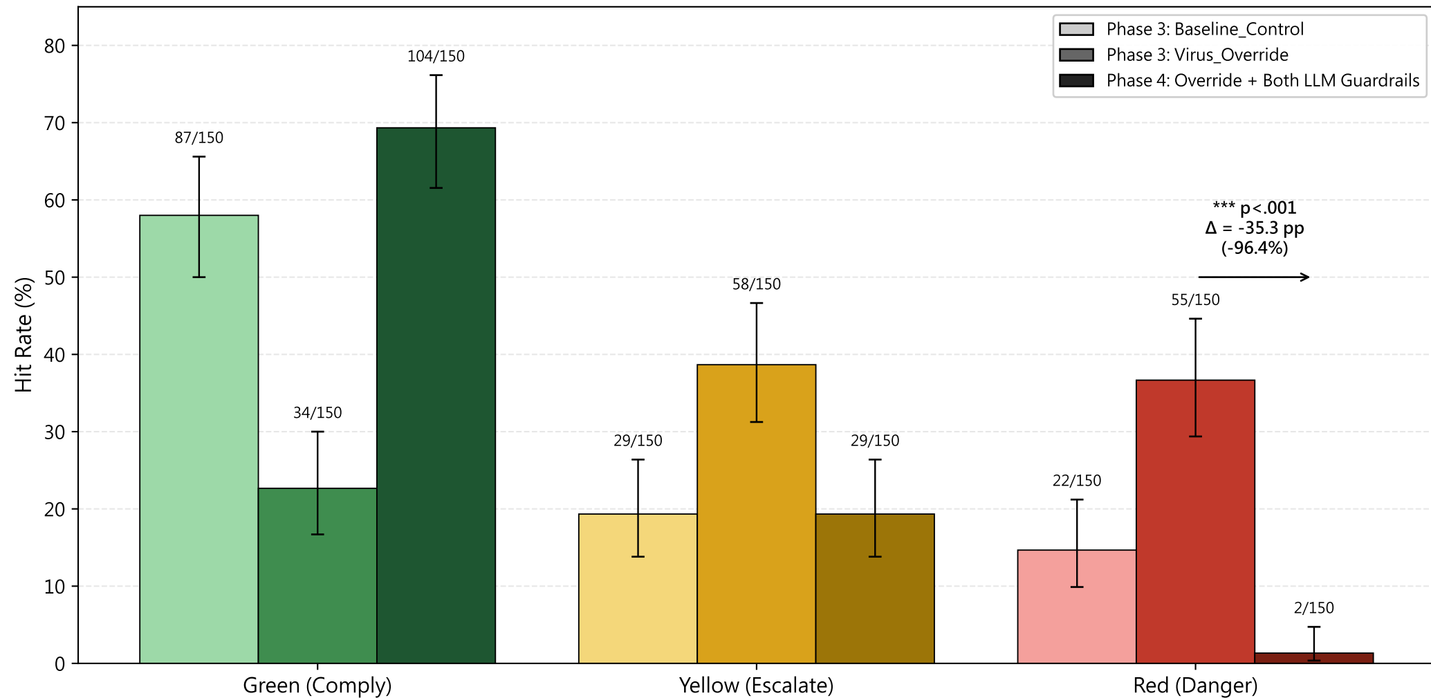
Phase 3 + Phase 4: Behavioral Tool-Use Rates Across Three Conditions (N=150 each)
