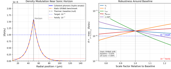
FIG. 4. Illustrative acoustic-model output. Left: Fractional density modulation |\delta\rho/\rho_0| versus distance from the horizon for coherent phonon injection in the hydrodynamic limit, the corresponding static GP/BdG benchmark, and the leading-order informational null prediction for the matched thermal control. The dashed blue line marks the target magnitude 10^{-6} ; the dotted red line marks the falsification threshold 10^{-7} . For the plotted baseline, the static GP/BdG response reduces the peak by 0.63% relative to the hydrodynamic estimate. Right: One-at-a-time \pm 25\% robustness scan of the peak signal A = \max_{|r-r_H| \leq L_{\text{coh}}} |\delta\rho/\rho_0| around the Gross-Pitaevskii-compatible baseline, for n_0 , \xi , L_{\text{coh}} , N_{\text{phonon}} , and c_s with \xi = \hbar/(\sqrt{2}mc_s) enforced for the c_s curve. Within the plotted range, the coherent signal stays above the falsification threshold and the static GP/BdG correction stays below 0.9%. Parameters: ^{87}\text{Rb} BEC, n_0 = 10^{14} \text{ cm}^{-3} , \rho_0 \approx 1.4 \times 10^{-5} \text{ kg/m}^3 , c_s \approx 1.7 \text{ mm/s} , \xi = 0.3 \mu\text{m} , r_H = 50 \mu\text{m} , L_{\text{coh}} = 10 \mu\text{m} , N_{\text{phonon}} = 10^3 .
