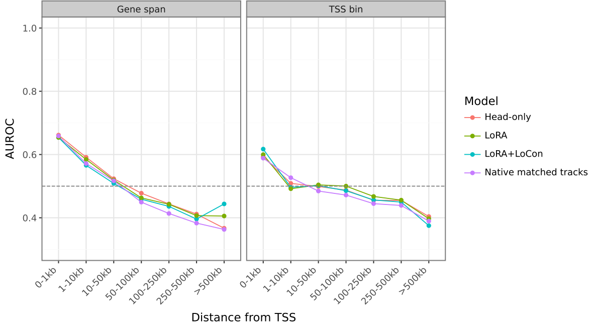
Figure 1: AUROC by distance from the TSS for TSS-bin and gene-span mutation effects. The dashed line is chance performance. Native matched tracks use the biologically defensible panel-specific selections in Table 4.
