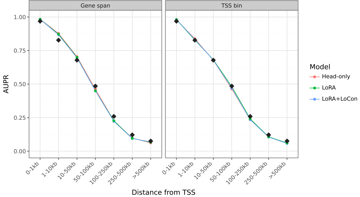
Figure 2: AUPR by distance from the TSS for TSS-bin and gene-span mutation effects. Black diamonds show the random-ranking reference, equal to the positive variant fraction in each distance bin.
