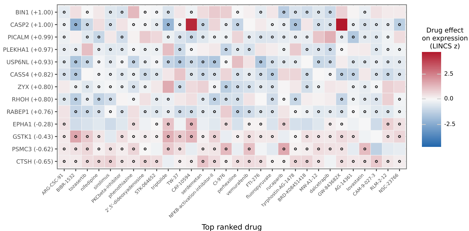
Top CPA/LINCS drug effects on ISOMIGA AD coloc genes
