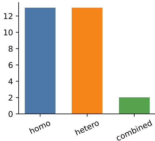
Retained rank
