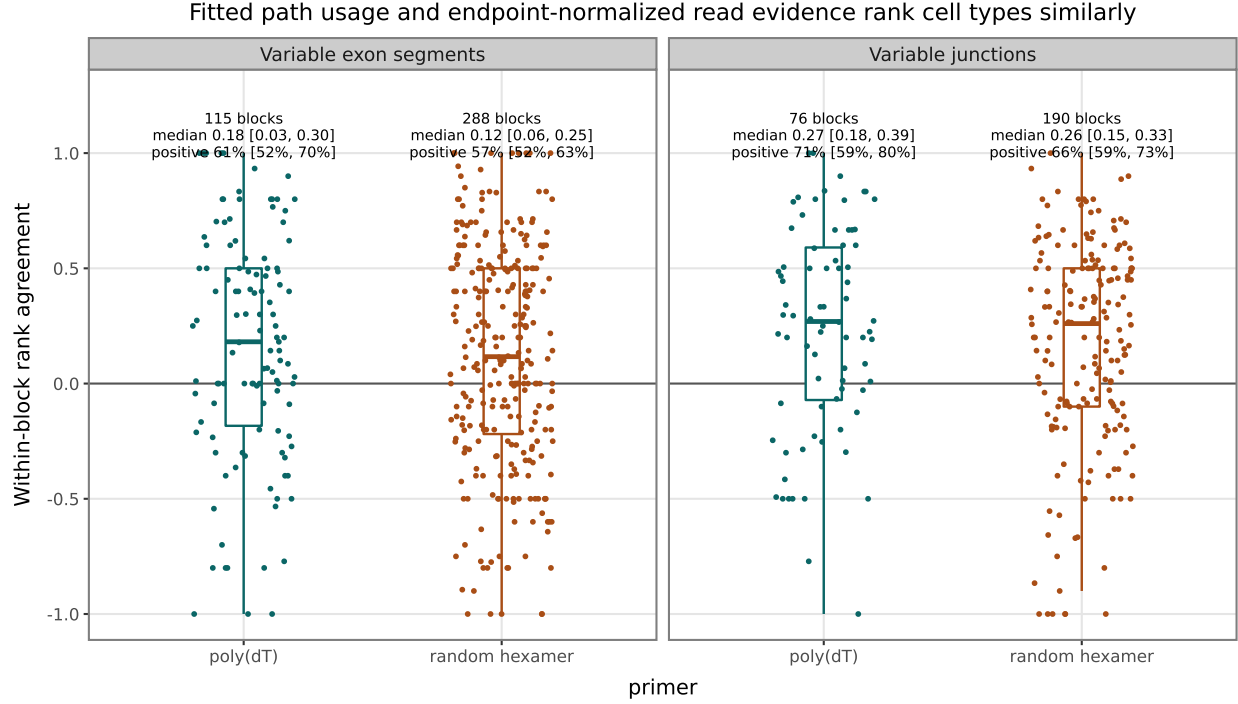
Figure 2: Agreement between weakly regularized fitted path usage and endpoint-normalized alignment evidence across significant omnibus blocks. Each point is one support-qualified block and averages within-feature Spearman correlations across cell types. Boxes show medians and interquartile ranges, annotations give block counts, bootstrap intervals for the median, and bootstrap intervals for the positive fraction, and the horizontal line marks no directional agreement. Significance is inherited from the production A_{\text{test}} = 64 omnibus analysis; fitted inclusion uses the separate A_{\text{report}} = 1 reporting refit and cannot alter discovery.
