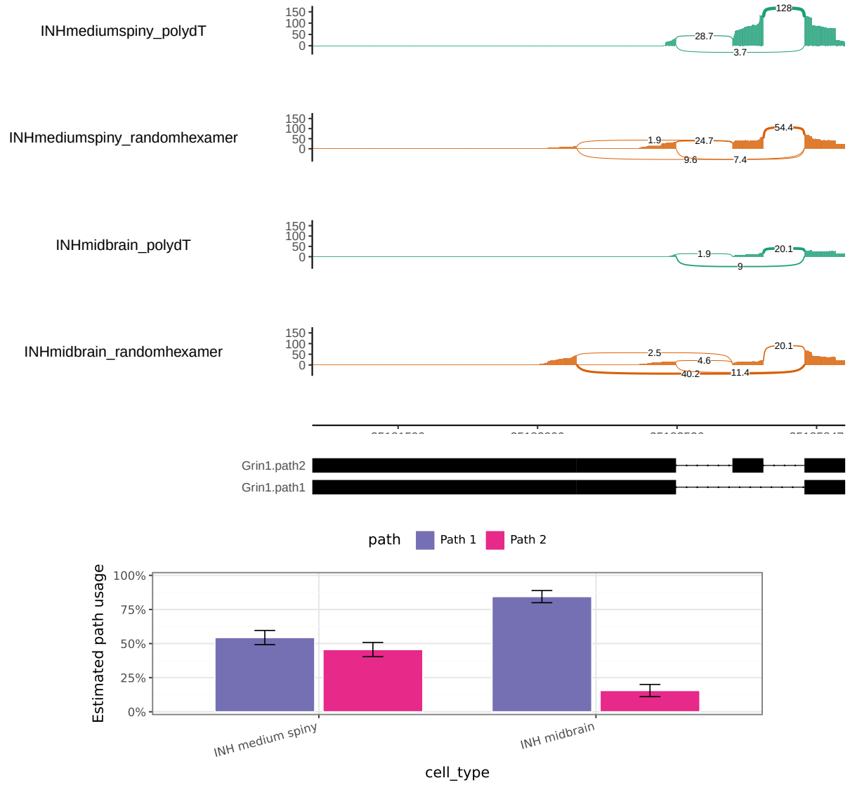
Figure 5: Primer-separated spliced-read support and fitted path usage for the Grin1 C1 cassette, block B3. INHmediumspiny and INHmidbrain denote medium-spiny and midbrain inhibitory cells. Track labels and normalization follow Figure 3; the lower panel shows A_{\text{report}} = 1 mean path proportions with standard errors across nine paired subjects.
