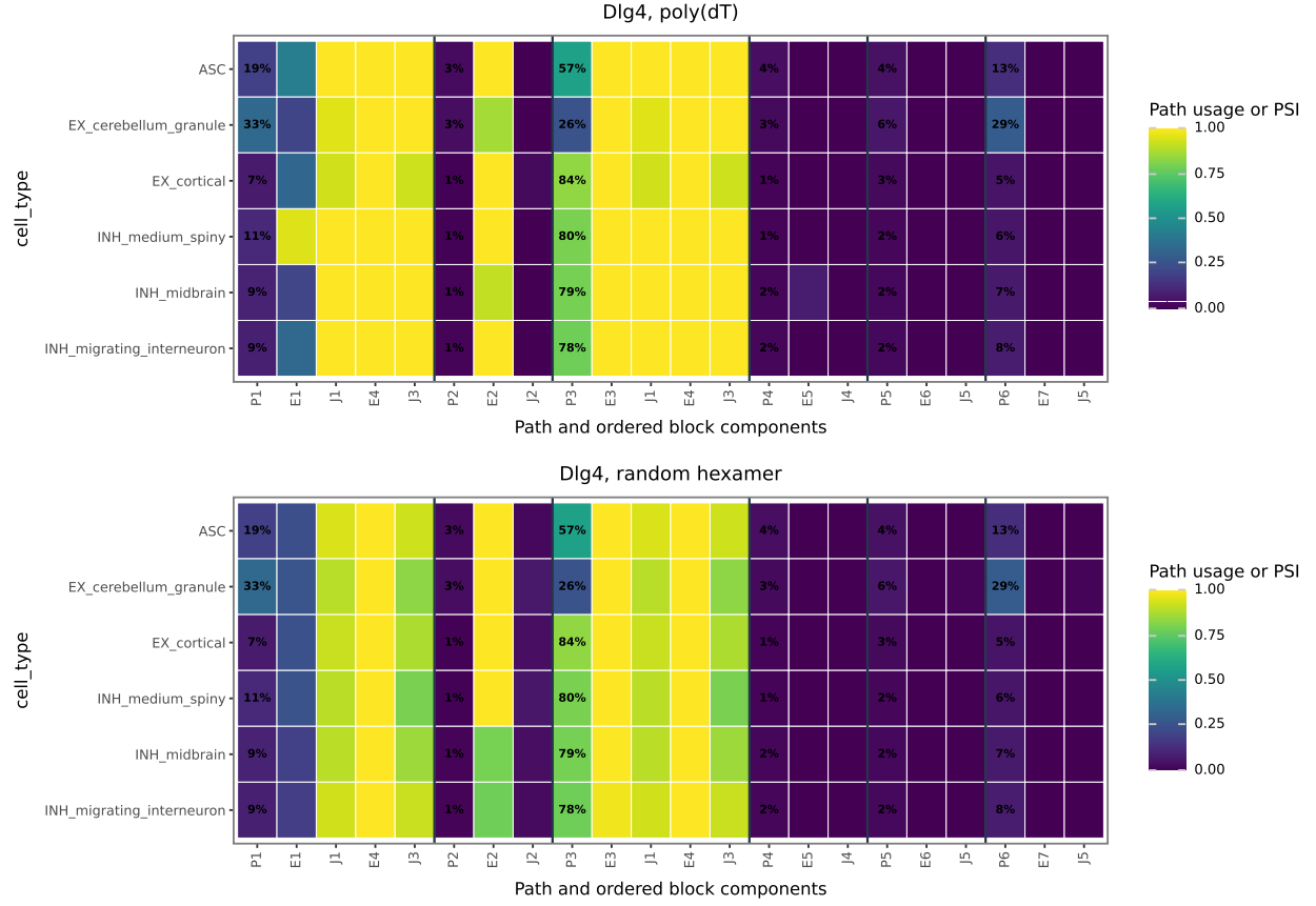
Figure 7: Second-largest weakly regularized dominant-path change, the six-path Dlg4 alternative-first-region block. Path 3 rises from 0.258 in cerebellar-granule excitatory cells to 0.836 in cortical excitatory cells. Definitions and panel order follow Figure 6.
