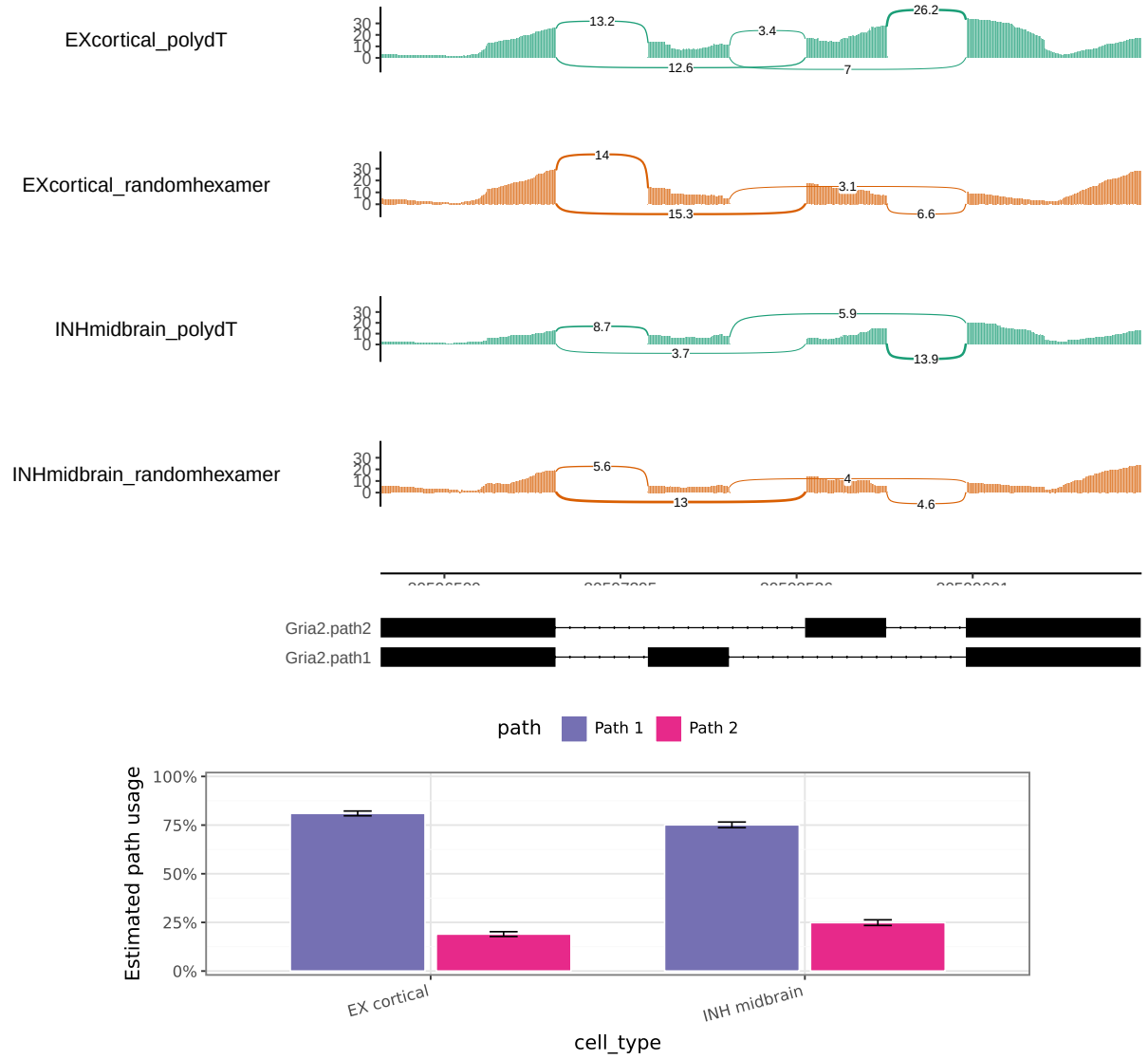
Figure 4: Primer-separated spliced-read support and fitted path usage for the mutually exclusive Gria2 flip/flop exons, block B1. EXcortical and INHmidbrain denote cortical excitatory and midbrain inhibitory cells. Track labels and normalization follow Figure 3; the lower panel shows A_{\text{report}} = 1 mean path proportions with standard errors across 39 paired subjects.
