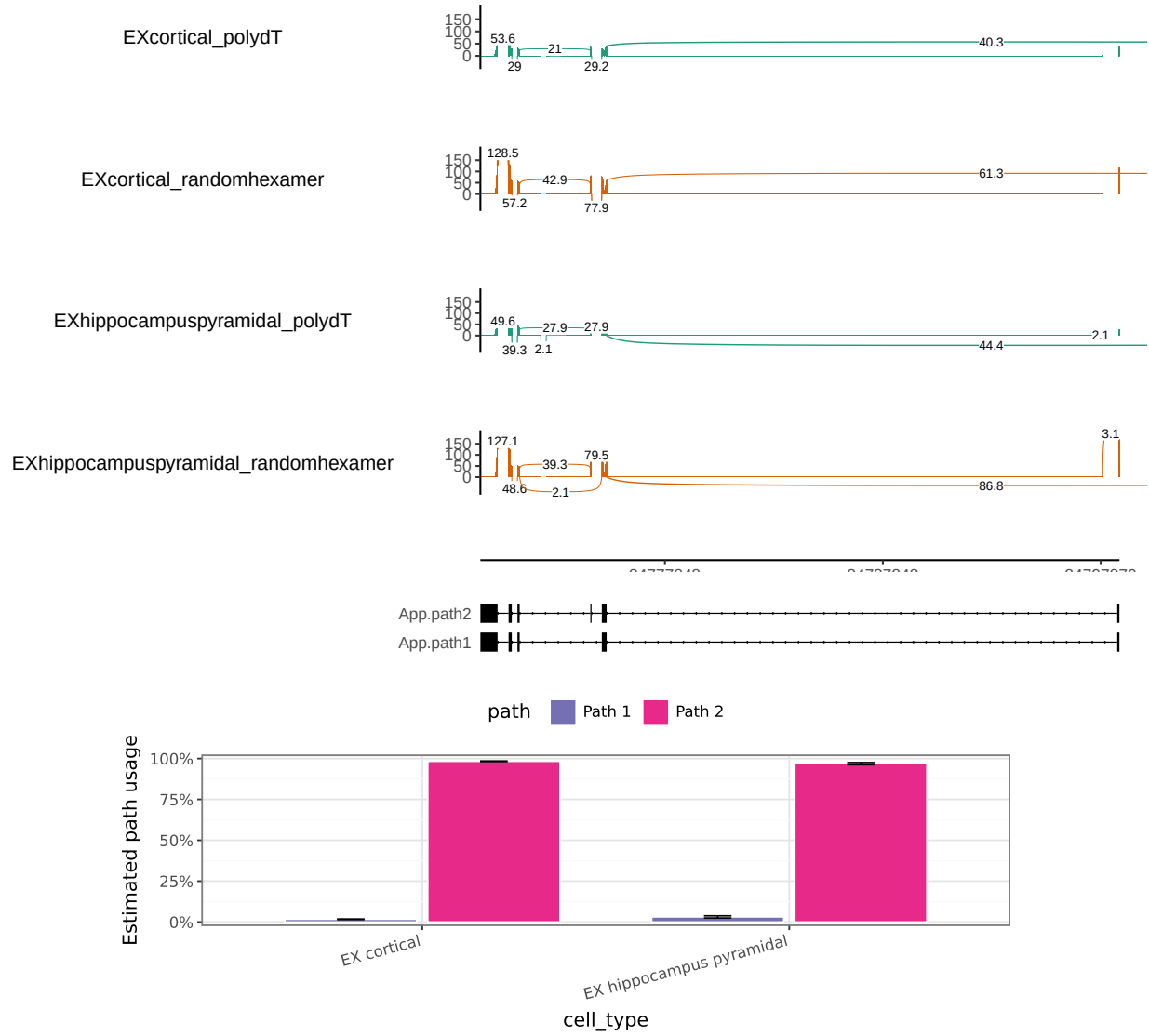
Figure 3: Primer-separated spliced-read support and fitted path usage for the App exon-15 cassette, block B3. EXcortical and EXhippocampuspyramidal denote cortical excitatory and hippocampal pyramidal cells. Teal and orange tracks are poly(dT) and random-hexamer half-cells. The lower panel shows A_{\text{report}} = 1 mean path proportions with standard errors across four paired subjects.
