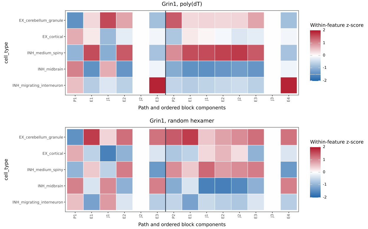
Figure 7: Path-ordered block evidence across all five cell types represented in the Grin1 omnibus fit, separated into poly(dT) and random-hexamer panels. Column definitions and scaling follow Figure 5.
