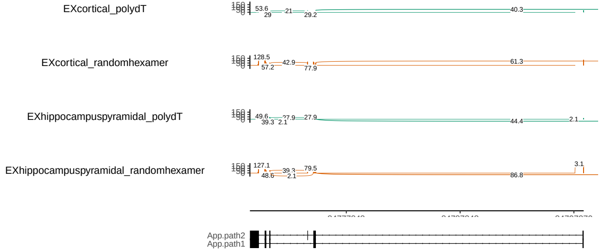
Figure 2: Primer-separated spliced-read support for the App exon-15 cassette, block B3. EXcortical and EXhippocampuspyramidal denote cortical excitatory and hippocampal pyramidal cells. Teal and orange tracks are poly(dT) and random-hexamer half-cells.
