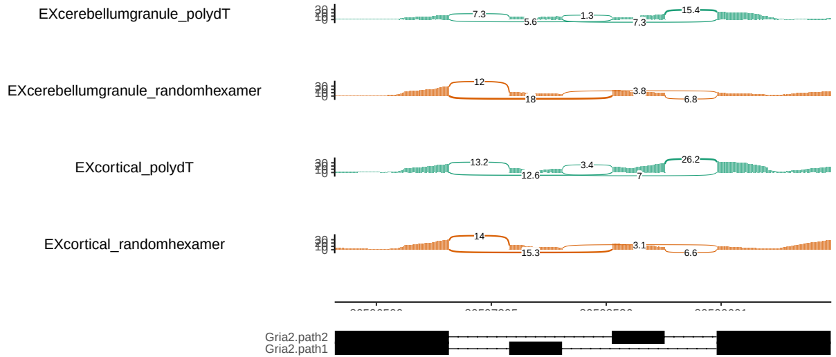
Figure 3: Primer-separated spliced-read support for the mutually exclusive Gria2 flip/flop exons, block B1. EXcerebellumgranule and EXcortical denote cerebellar-granule and cortical-excitatory cells. Track labels and normalization follow Figure 2.
