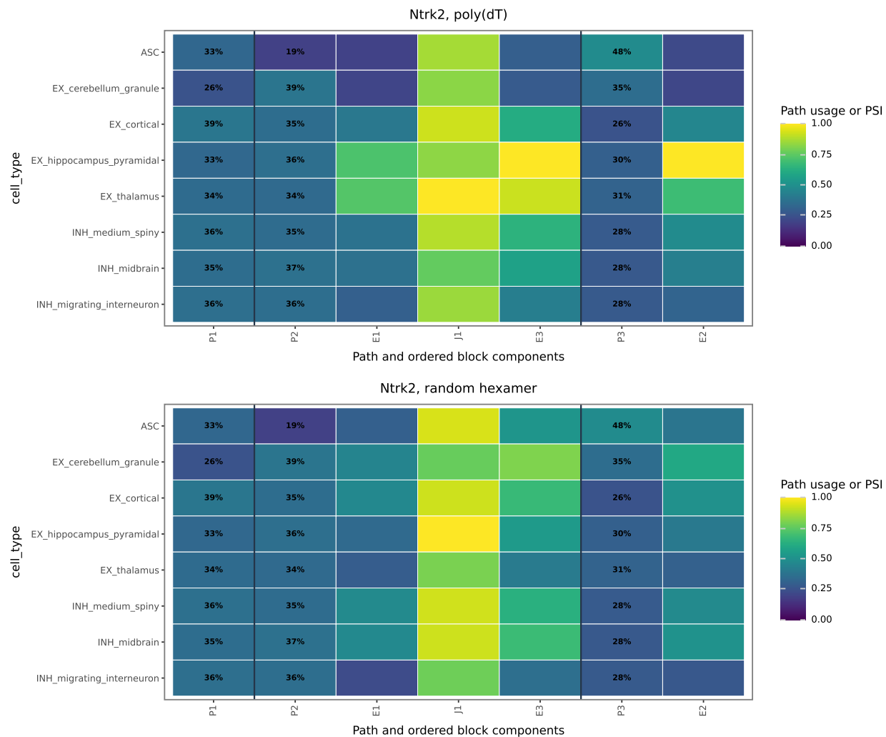
Figure 7: Third-largest eligible fitted dominant-path change, the three-path Ntrk2 alternative-first-region block. Path 3 rises from 0.255 in cortical excitatory cells to 0.480 in astrocytes. Definitions and panel order follow Figure 5.
