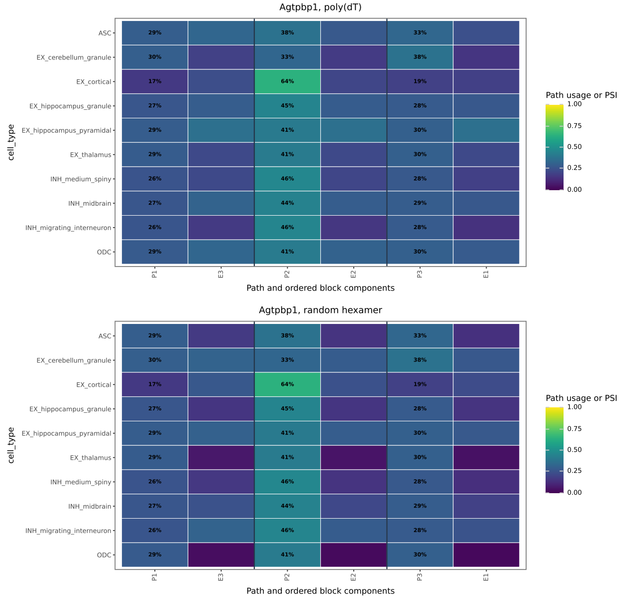
Figure 5: Strongest fitted dominant-path change, the Agtbbp1 alternative-first-region block. Path 2 rises from 0.326 in cerebellar-granule excitatory cells to 0.639 in cortical excitatory cells. P columns show joint-model fitted path usage; E and J columns show primer-specific exon and junction PSI.
