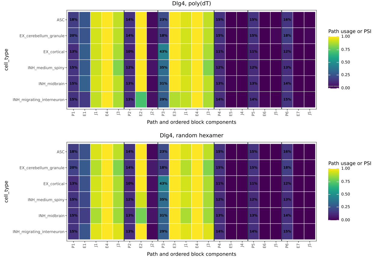
Figure 6: Second-largest eligible fitted dominant-path change, the six-path Dlg4 alternative-first-region block. Path 3 rises from 0.179 in cerebellar-granule excitatory cells to 0.430 in cortical excitatory cells. Definitions and panel order follow Figure 5.
