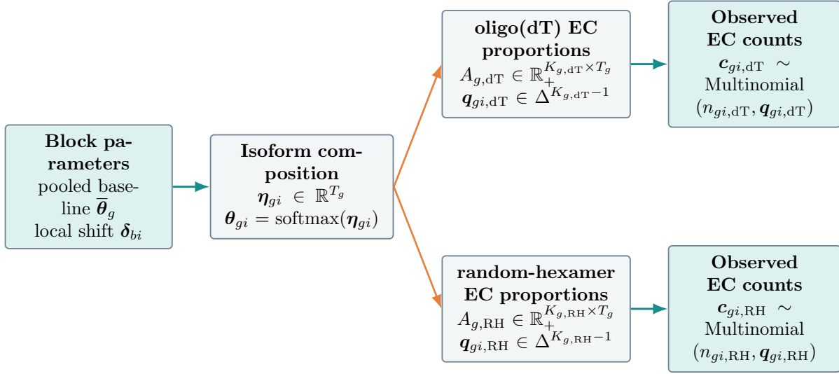
Figure 5: Generative flow for the deprecated global EC GLMM for gene g = g(b) and pseudobulk i . The two primer maps share the same latent global isoform composition.
