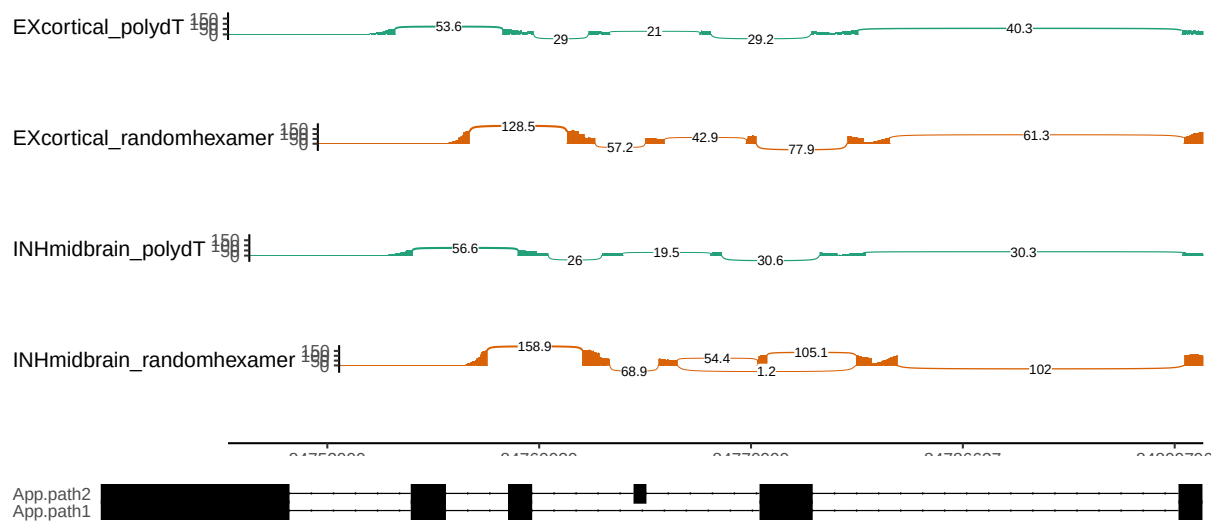
Figure 2: Primer-separated spliced-read support for the App exon-15 cassette, block B3. EXcortical and INHmidbrain denote cortical excitatory and midbrain inhibitory cells. Teal and orange tracks are poly(dT) and random-hexamer half-cells.
