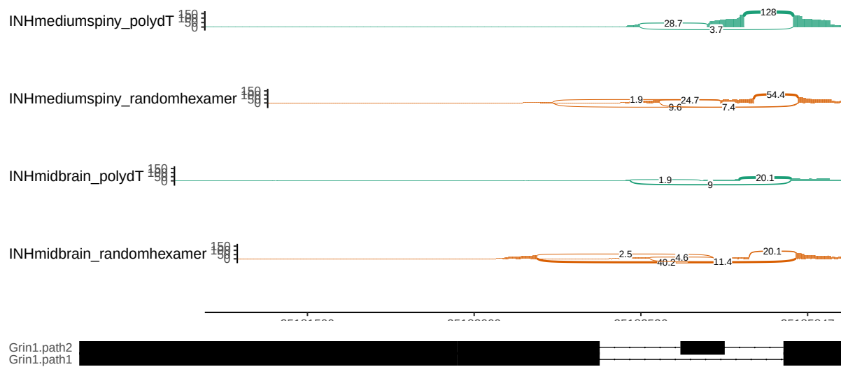
Figure 4: Primer-separated spliced-read support for the Grin1 C1 cassette, block B3. INHmediumspiny and INHmidbrain denote medium-spiny and midbrain inhibitory cells. Track labels and normalization follow Figure 2.
