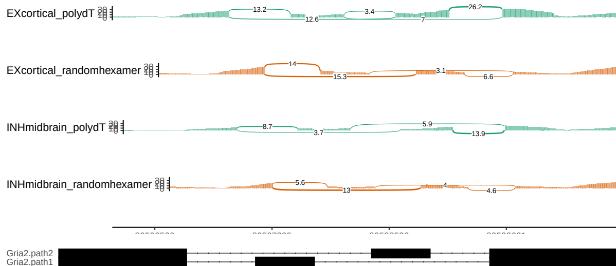
Figure 3: Primer-separated spliced-read support for the mutually exclusive Gria2 flip/flop exons, block B1. Track labels and normalization follow Figure 2.
