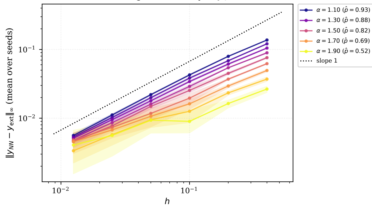
(b) fPINN convergence to analytic y_{\text{ext}} (95% CI)
