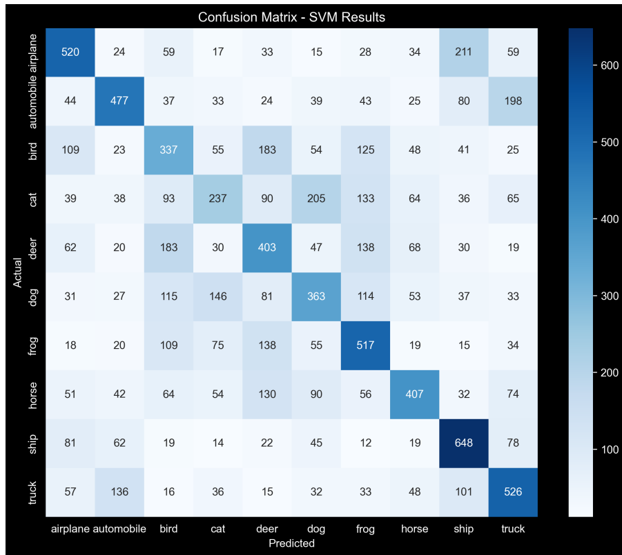
Figure 5: Confusion Matrix for the SVM Model on CIFAR-10
