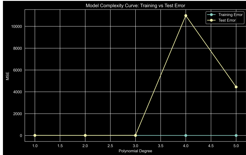
Figure 2: Model Complexity Curve: Training vs. Test MSE
