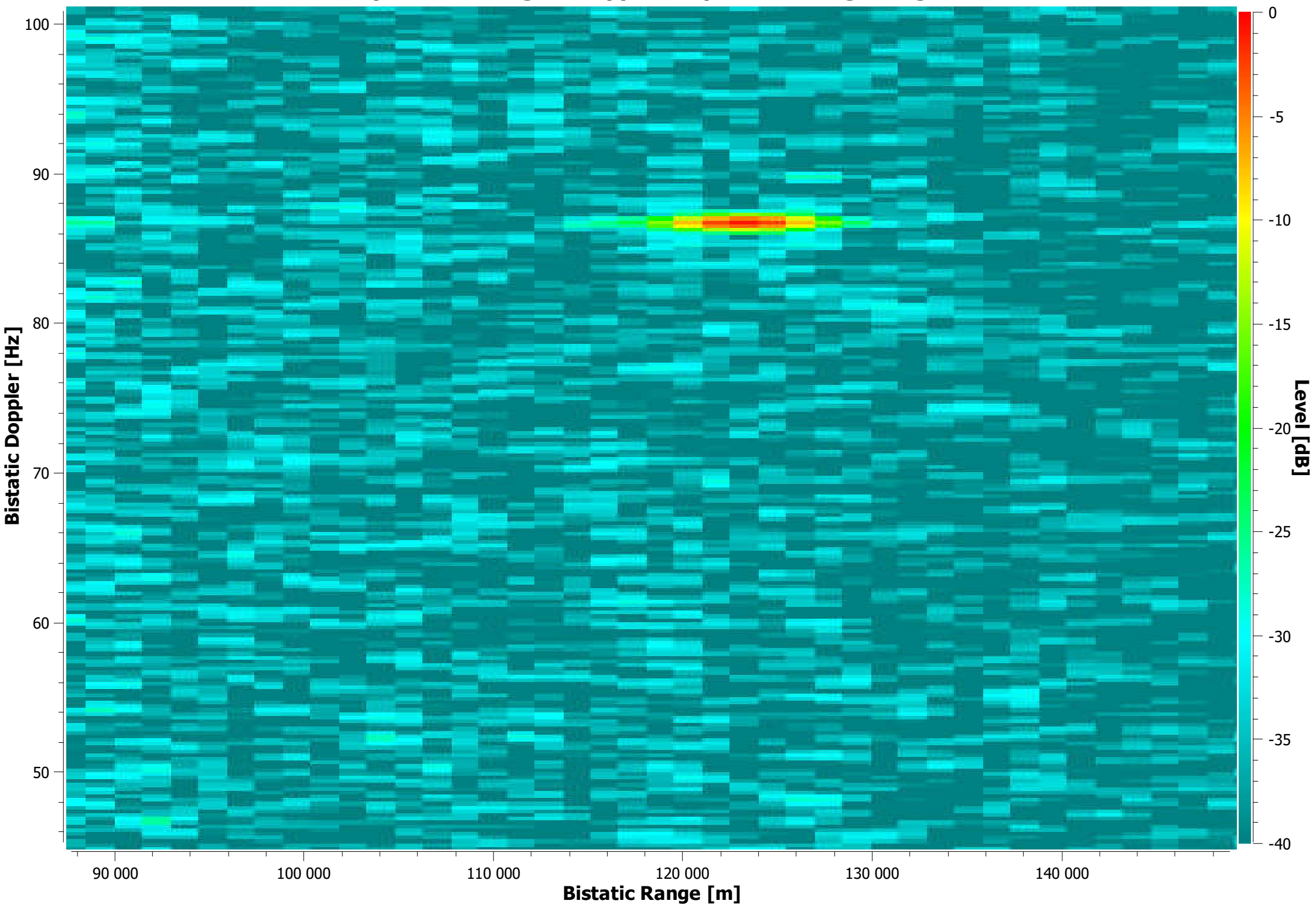
Amplitude / Range / Doppler Map: CleanSingleTarget.ard
