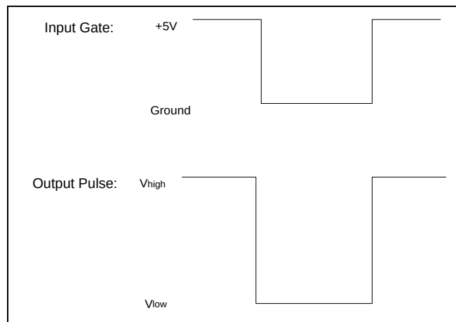
Generating a Negative Pulse With The PVX-4151 4.6
