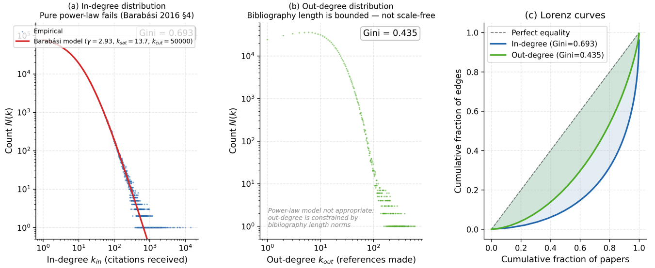
APS Citation Graph: Structural Properties (709,803 papers, 9,833,191 edges)
