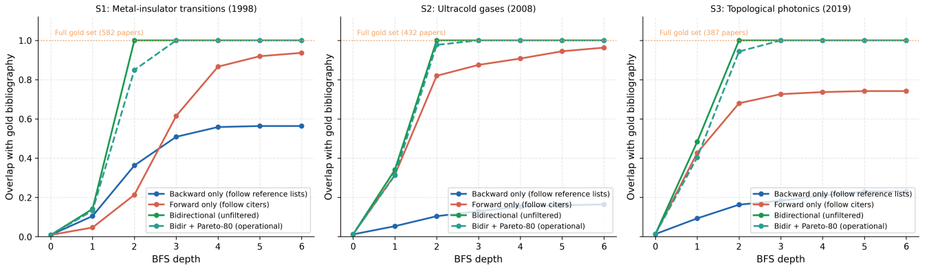
Figure 2: BFS overlap with gold bibliography by traversal direction (oracle seeds: k = 5 drawn from gold bibliography — upper bound on cold-start performance; dashed line = Pareto-80 operational default). Bidirectional traversal is necessary — forward-only misses foundational work, backward-only misses later work. The Pareto-80 curve closely tracks unfiltered bidirectional coverage, confirming hub suppression does not impede topical reachability at the depths used in practice.
