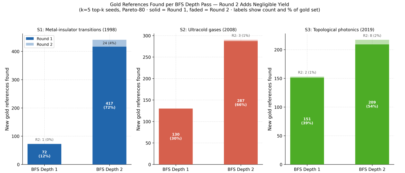
Figure 4: Screen yield collapse by BFS depth. Stacked bars show gold papers recovered per depth pass, split by round (solid = Round 1, lighter = Round 2). Yield collapses sharply at depth 2 across all three surveys. Round 2 adds a small insurance increment (1–4%); the stopping criterion fires reliably at depth 2 without parameter sensitivity.
