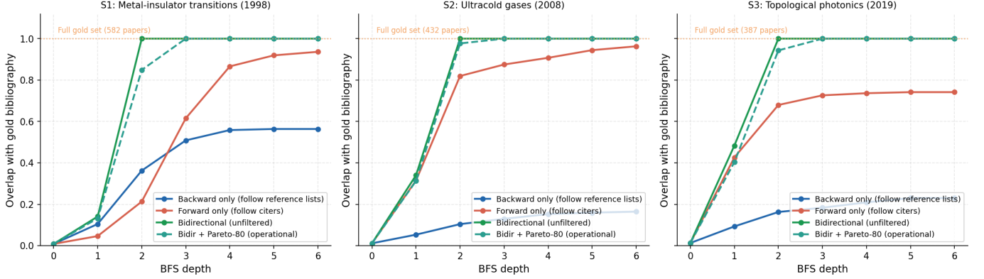
Fig. 2: BFS overlap with gold bibliography by traversal direction (oracle seeds: k = 5 drawn from gold bibliography — upper bound on cold-start performance; dashed line = Pareto-80 operational default). Bidirectional traversal is necessary — forward-only misses foundational work, backward-only misses later work. The Pareto-80 curve closely tracks unfiltered bidirectional coverage, confirming hub suppression does not impede topical reachability at the depths used in practice.
