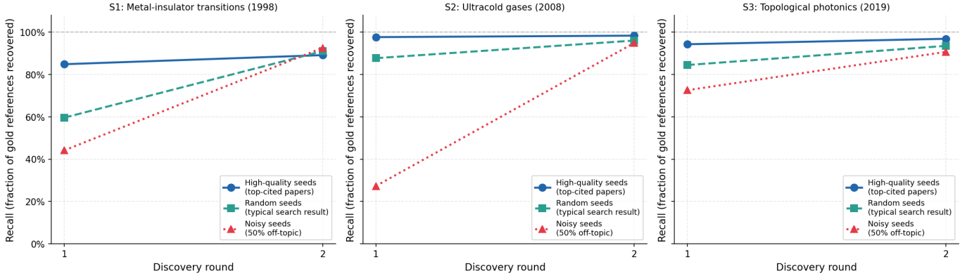
Fig. 5: Cold-start recall per round at k = 5 , for top- k , random, and contaminated seeds across all three surveys. Round 1 dominates; round 2 provides a small but consistent insurance increment. All seed types converge to \geq 90\% by round 2.
