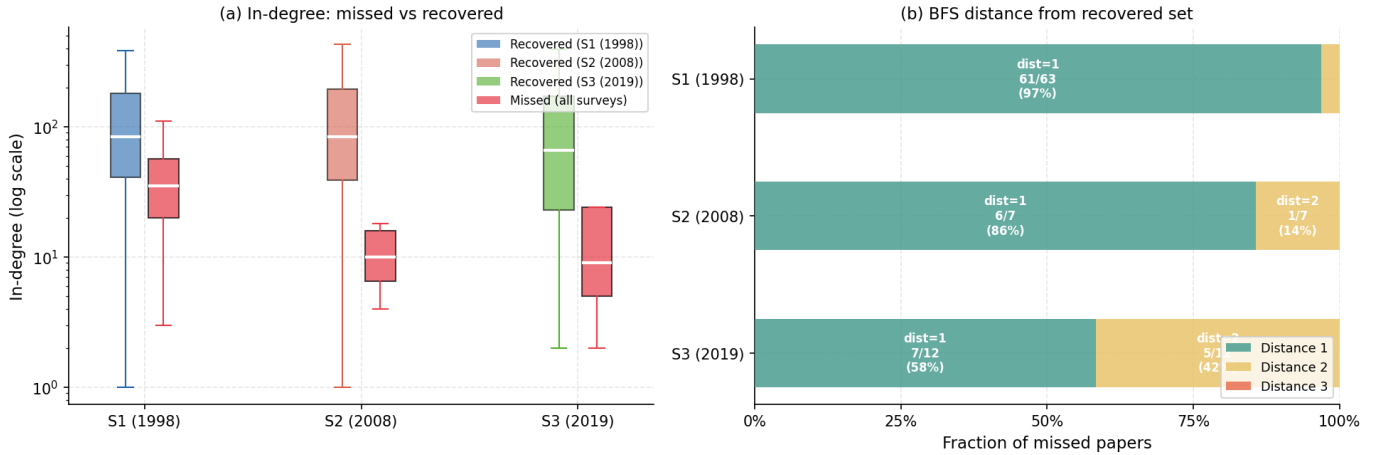
Fig. 7: Anatomy of the residual coverage gap. Left: In-degree distribution of missed vs recovered papers (log scale) across all three surveys. Missed papers cluster at the low-in-degree tail. Right: BFS distance from the recovered set to missed papers. Nearly all misses are within 2 hops — structurally adjacent but not reached before yield collapse.
