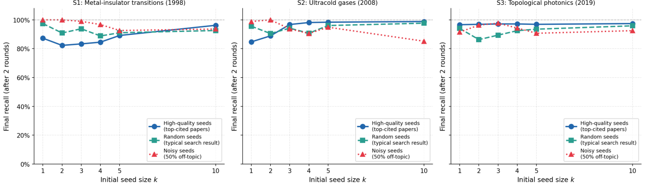
Fig. 6: Final recall vs seed size k \in \{1, 2, 3, 4, 5, 10\} (after two rounds) for all seed types and surveys. Top- k recall dips at k = 2 because nearest-neighbour seeds share backward neighbourhoods; contaminated recall declines with k because each off-topic seed opens a new traversal frontier. Both effects resolve by round 2.
