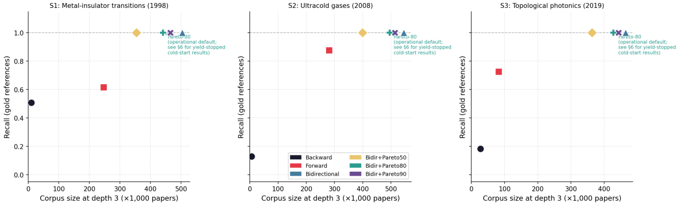
Fig. 3: Coverage–cost trade-off: recall vs corpus size at BFS depth 3 . All strategies shown for each survey. Pareto-filtered bidirectional traversal (operational default) achieves near-identical recall to unfiltered bidirectional at substantially reduced corpus size.
