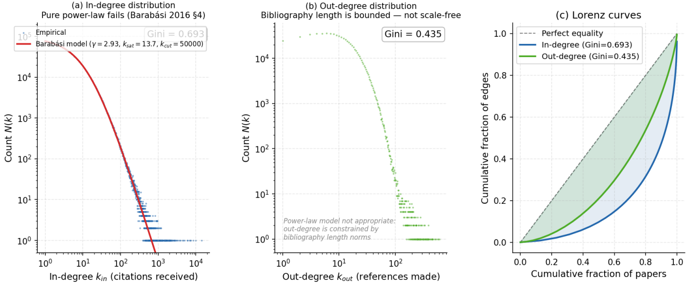
Fig. 1: Degree distributions of the APS citation graph. In-degree (citations received) is heavy-tailed; out-degree (references made) is bounded. The asymmetry motivates why forward traversal explodes while backward traversal stays local.
