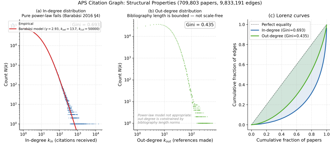
Fig. 1. Degree distributions of the APS citation graph. In-degree (citations received) is heavy-tailed; out-degree (references made) is bounded. The asymmetry motivates why forward traversal explodes while backward traversal stays local.
