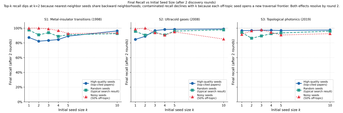
Fig. 6. Final recall vs seed size k \in \{1, 2, 3, 4, 5, 10\} (after two rounds) for all seed types and surveys. Top- k recall dips at k = 2 because nearest-neighbour seeds share backward neighbourhoods; contaminated recall declines with k because each off-topic seed opens a new traversal frontier. Both effects resolve by round 2.
