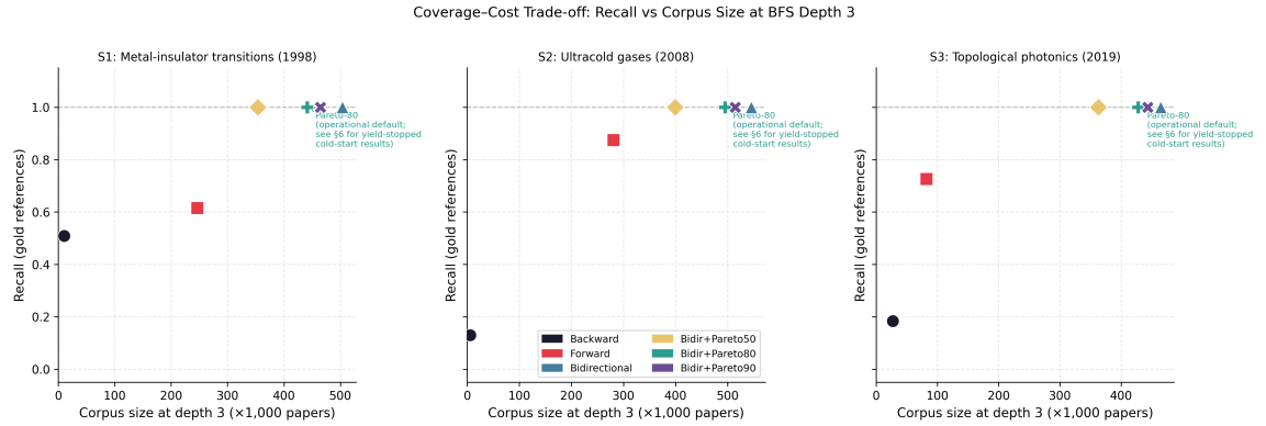
Fig. 3. Coverage-cost trade-off: recall vs corpus size at BFS depth 3. All strategies shown for each survey. Pareto-filtered bidirectional traversal (operational default) achieves near-identical recall to unfiltered bidirectional at substantially reduced corpus size.
