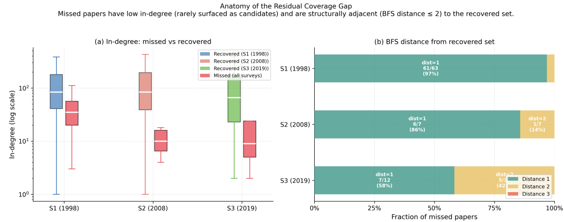
Fig. 7. Anatomy of the residual coverage gap. Left: In-degree distribution of missed vs recovered papers (log scale) across all three surveys. Missed papers cluster at the low-in-degree tail. Right: BFS distance from the recovered set to missed papers. Nearly all misses are within 2 hops — structurally adjacent but not reached before yield collapse.
