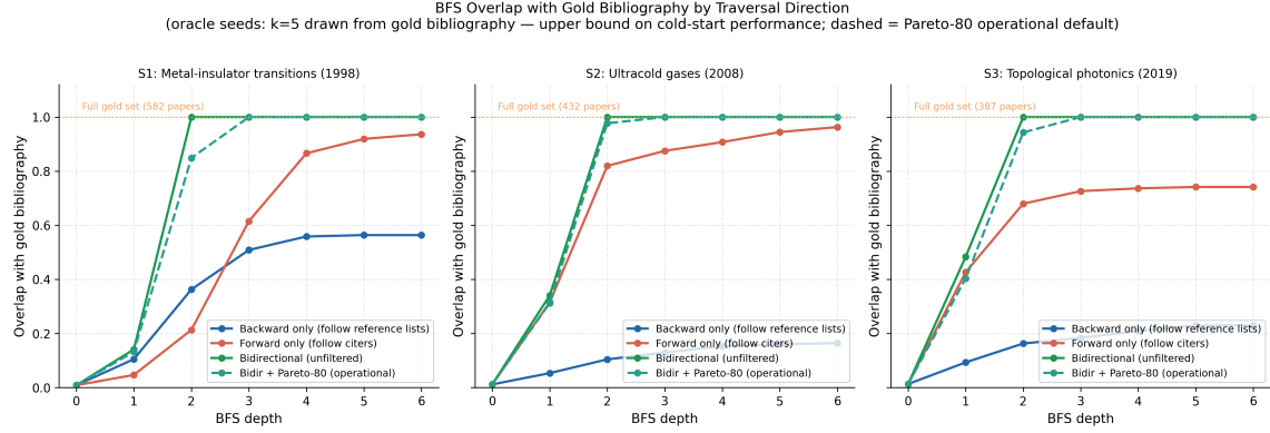
Fig. 2. BFS overlap with gold bibliography by traversal direction (oracle seeds: k = 5 drawn from gold bibliography — upper bound on cold-start performance; dashed line = Pareto-80 operational default). Bidirectional traversal is necessary — forward-only misses foundational work, backward-only misses later work. The Pareto-80 curve closely tracks unfiltered bidirectional coverage, confirming hub suppression does not impede topical reachability at the depths used in practice.
