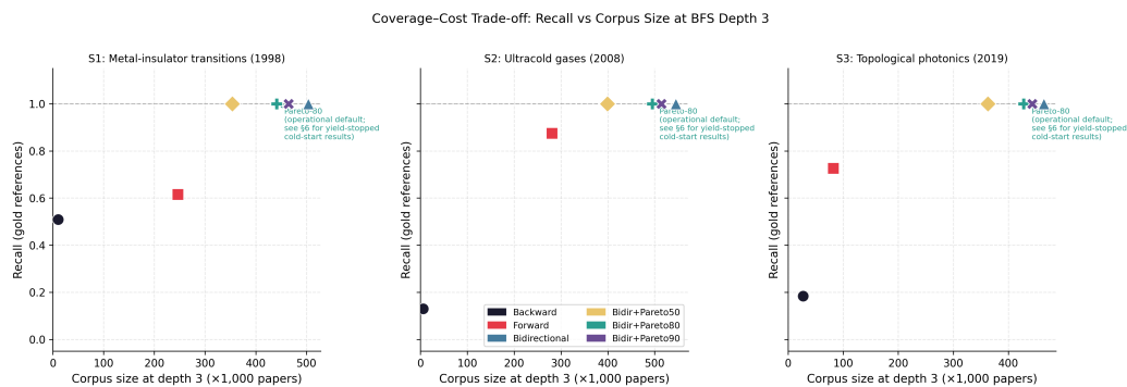
Figure 3: Coverage-cost trade-off: recall vs corpus size at BFS depth 3. All strategies shown for each survey. Pareto-filtered bidirectional traversal (operational default) achieves near-identical recall to unfiltered bidirectional at substantially reduced corpus size.
