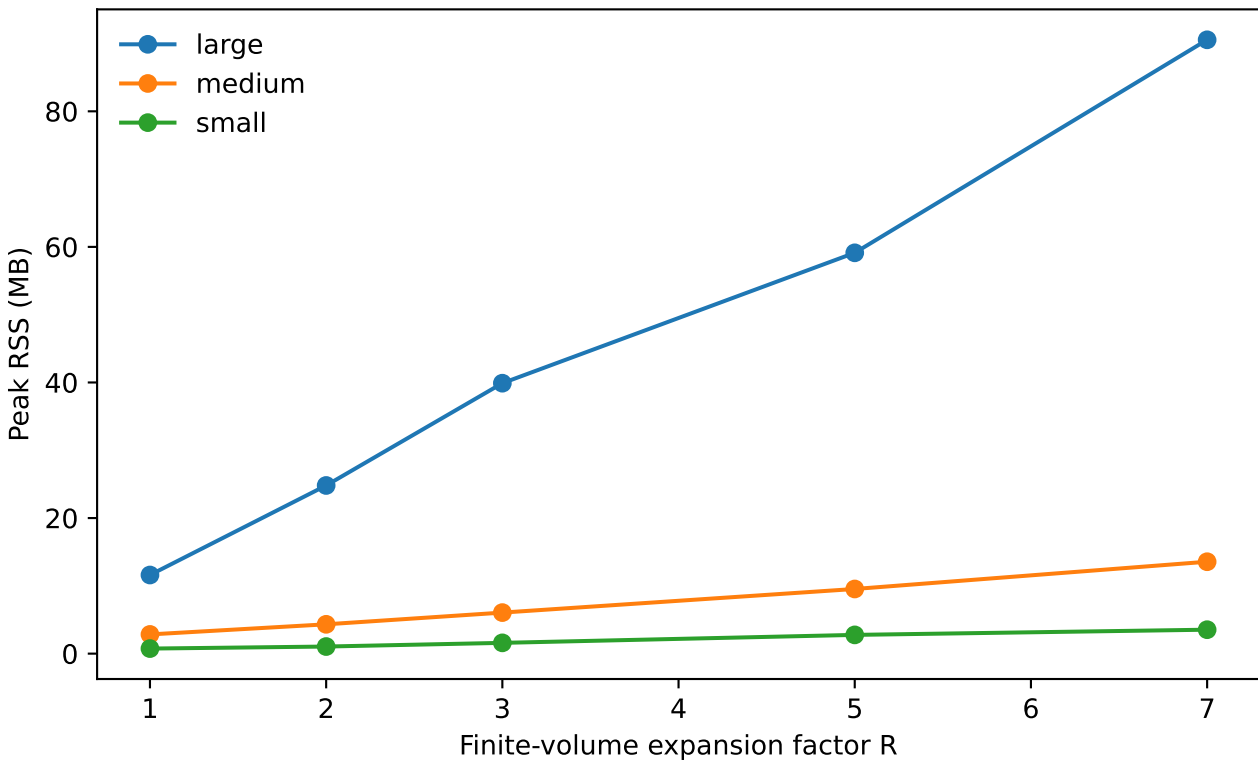
Approximate memory scaling
