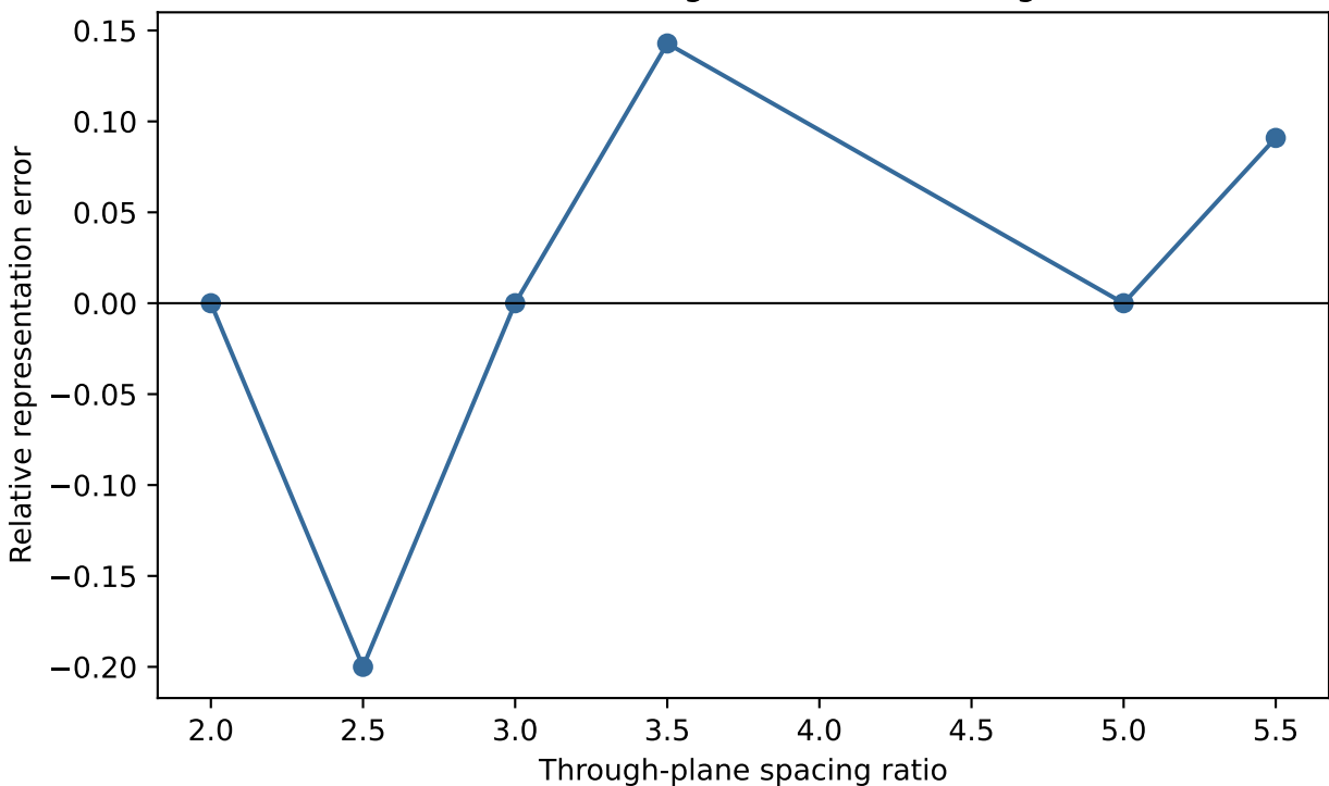
Finite-volume rounding error for non-integer ratios
