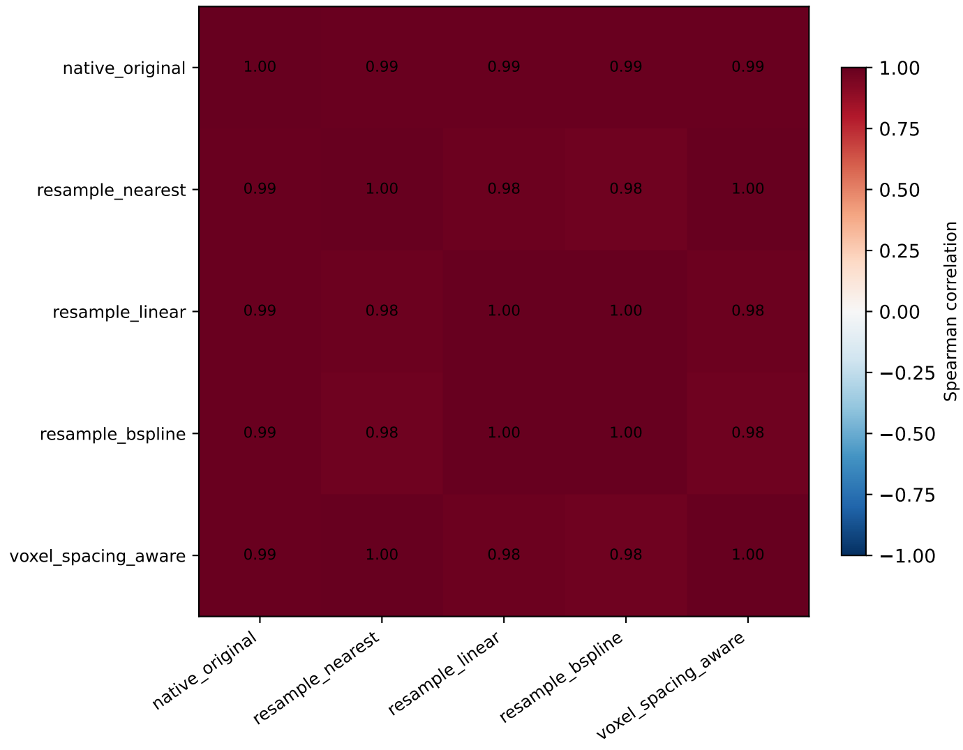
Similarity of extraction strategies across synthetic anisotropy settings
