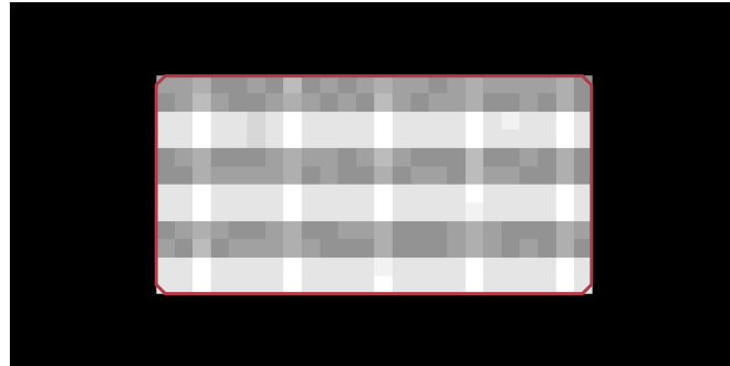
Sagittal
