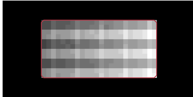
Coronal
