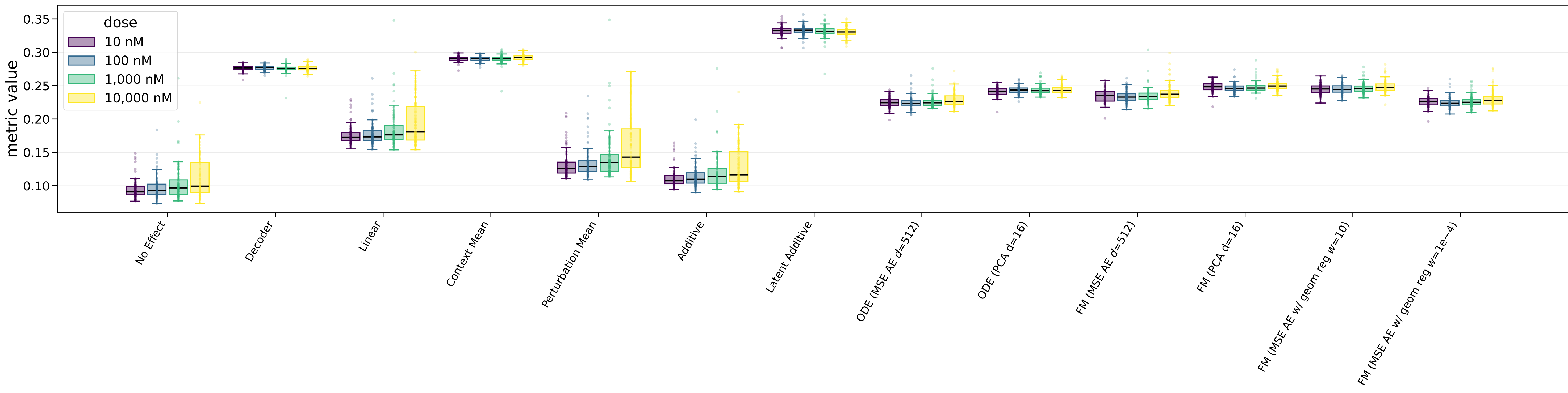
mean gene W_1 by model and dose ( \downarrow )
