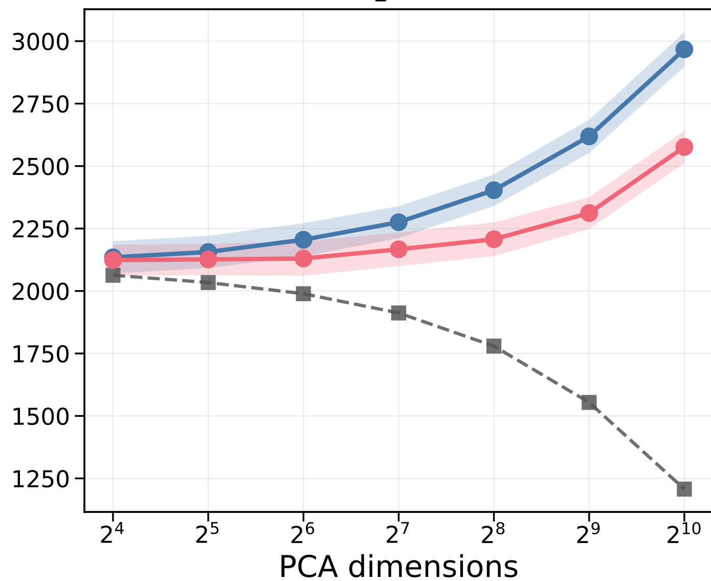
W_2^2 ( \downarrow )
