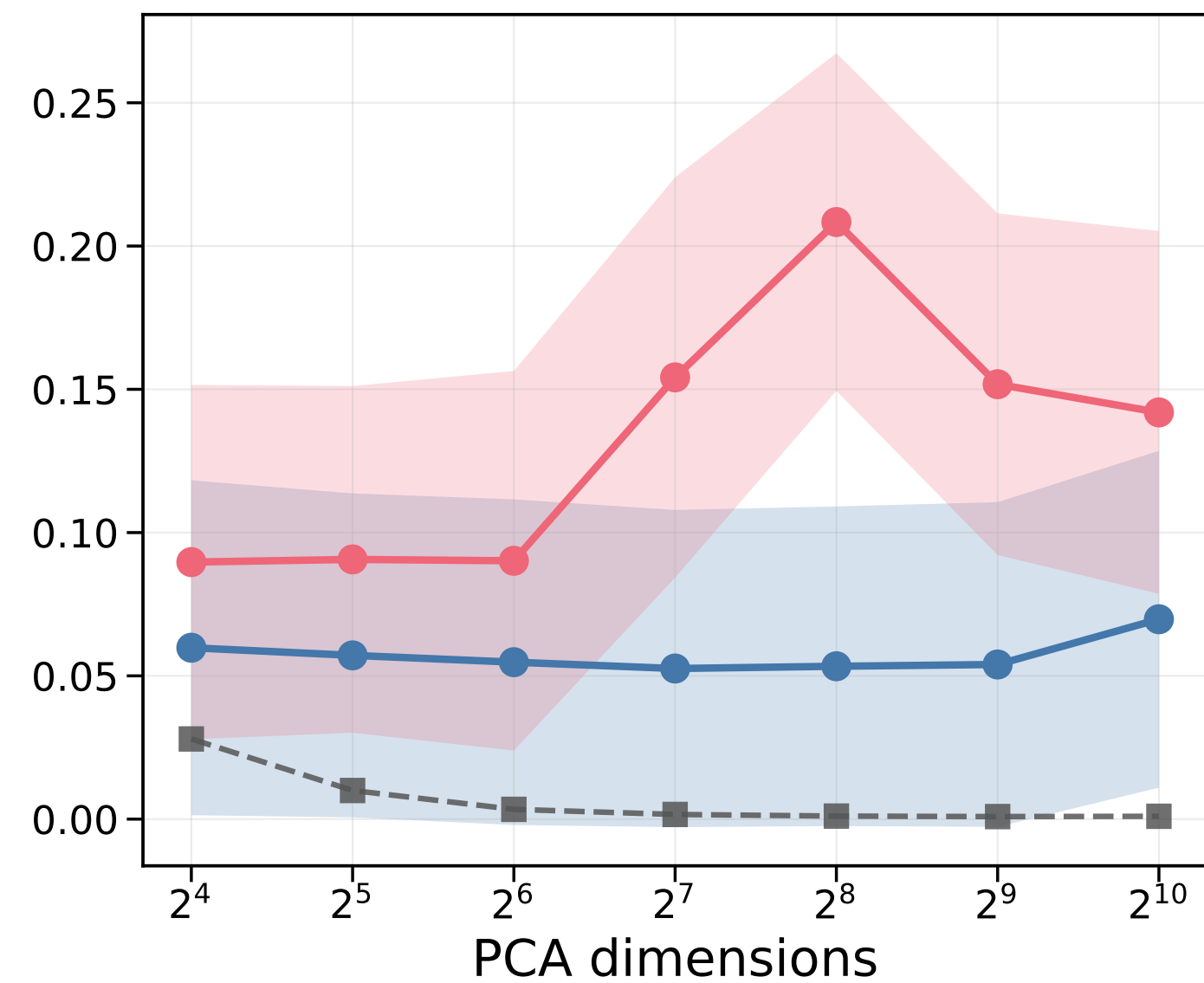
MMD ( \downarrow )
