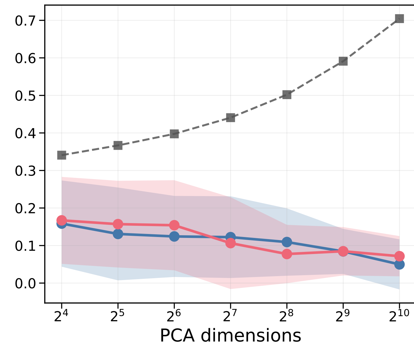
cosine logFC ( \uparrow )
