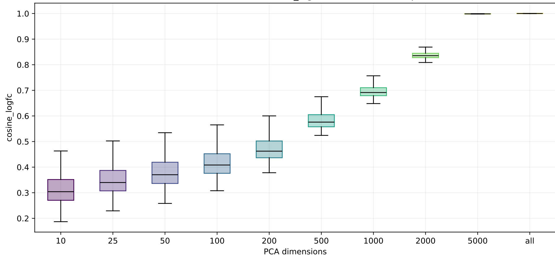
PCA theoretical limit: cosine_logfc distribution (test split)
