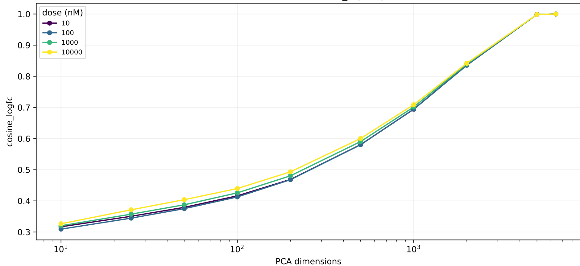
PCA theoretical limit: cosine_logfc by dose
