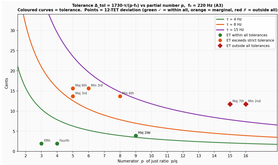
Figure 3: Tolerance half-width \Delta_{\text{tol}} = 1730\tau/(p \cdot f_0) as a function of the partial number p at f_0 = 220 Hz. Coloured curves show three threshold values. Interval points show their 12-TET deviations: green = ET within all tolerances, orange = ET exceeds strict tolerance, red = ET outside all tolerances.
