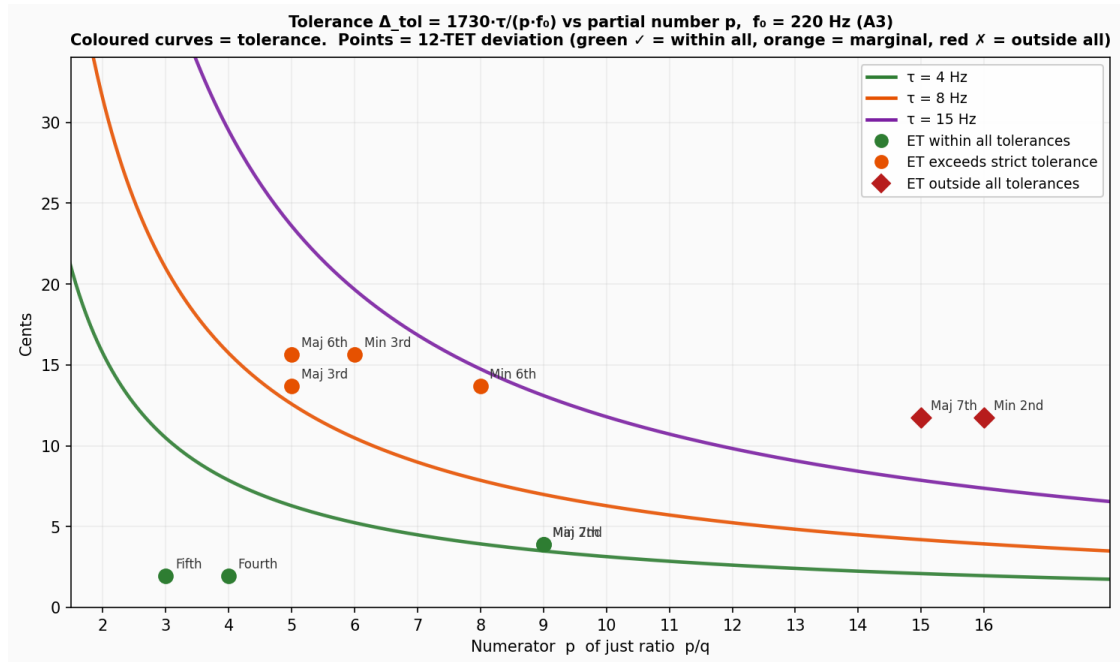
Figure 3: Tolerance half-width \Delta_{\text{tol}} = 1730\tau/(p \cdot f_0) as a function of the partial number p at f_0 = 220 Hz. Coloured curves show three threshold values. Interval points show their 12-TET deviations: green = ET within all tolerances, orange = ET exceeds strict tolerance, red = ET outside all tolerances.
