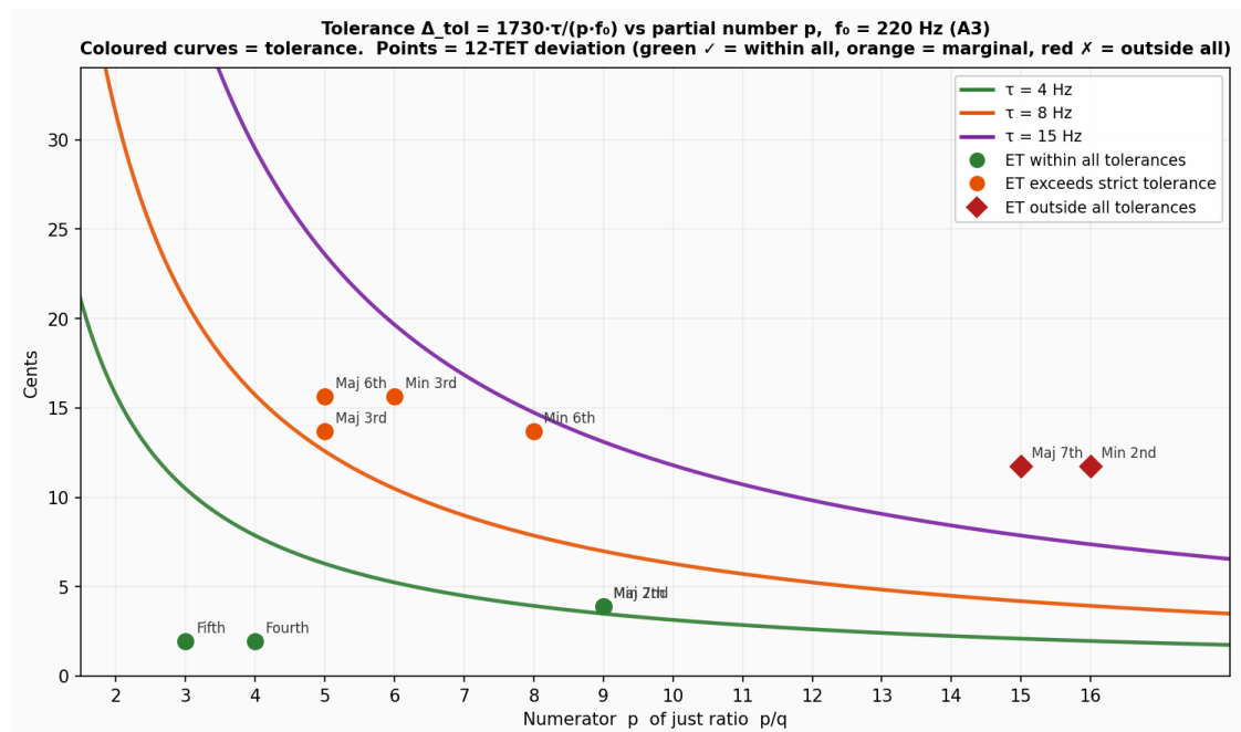
Figure 3: Tolerance half-width \Delta_{tol} = 1730\tau/(p \cdot f_0) as a function of the partial number p at f_0 = 220 Hz. Coloured curves show three threshold values. Interval points show their 12-TET deviations: green = ET within all tolerances, orange = ET exceeds strict tolerance, red = ET outside all tolerances.
