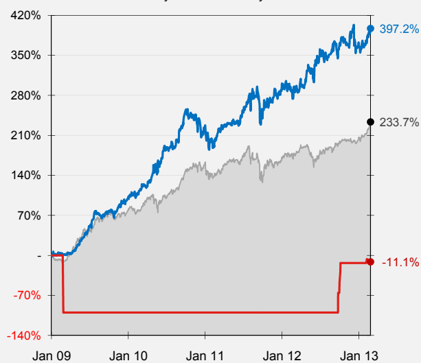
Closing Price*, Jakarta Composite Index (IHSG) and Consumer Goods Industry Index January 2009 - February 2013
