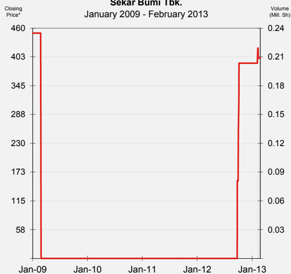
Closing Price* and Trading Volume Sekar Bumi Tbk. January 2009 - February 2013
