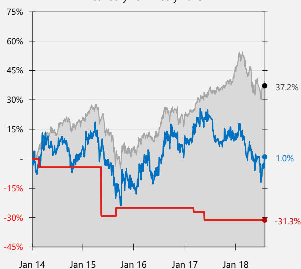
Closing Price*, Jakarta Composite Index (IHSG) and Miscellaneous Industry Index January 2014 - July 2018
