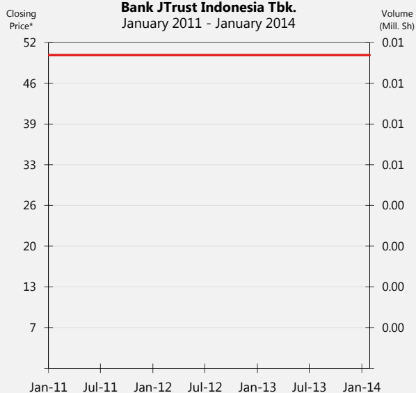
Closing Price*, Jakarta Composite Index (IHSG) and Finance Index January 2011 - January 2014
