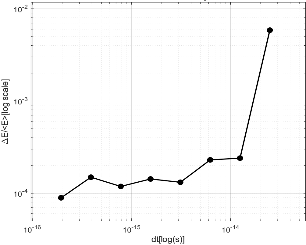
\Delta E / \langle E \rangle vs timestep
