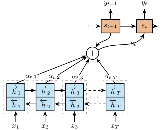
Figure 36: RNN with attention: a bidirectional encoder produces hidden states \vec{h}_j ; alignment weights \alpha_{t,j} combine them into the context vector c_t that feeds the decoder state s_t generating y_t .
