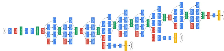
Figure 23: GoogLeNet architecture.
