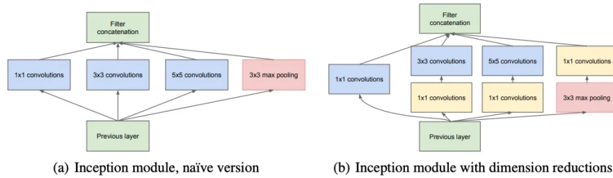
Figure 24: Inception Module.
