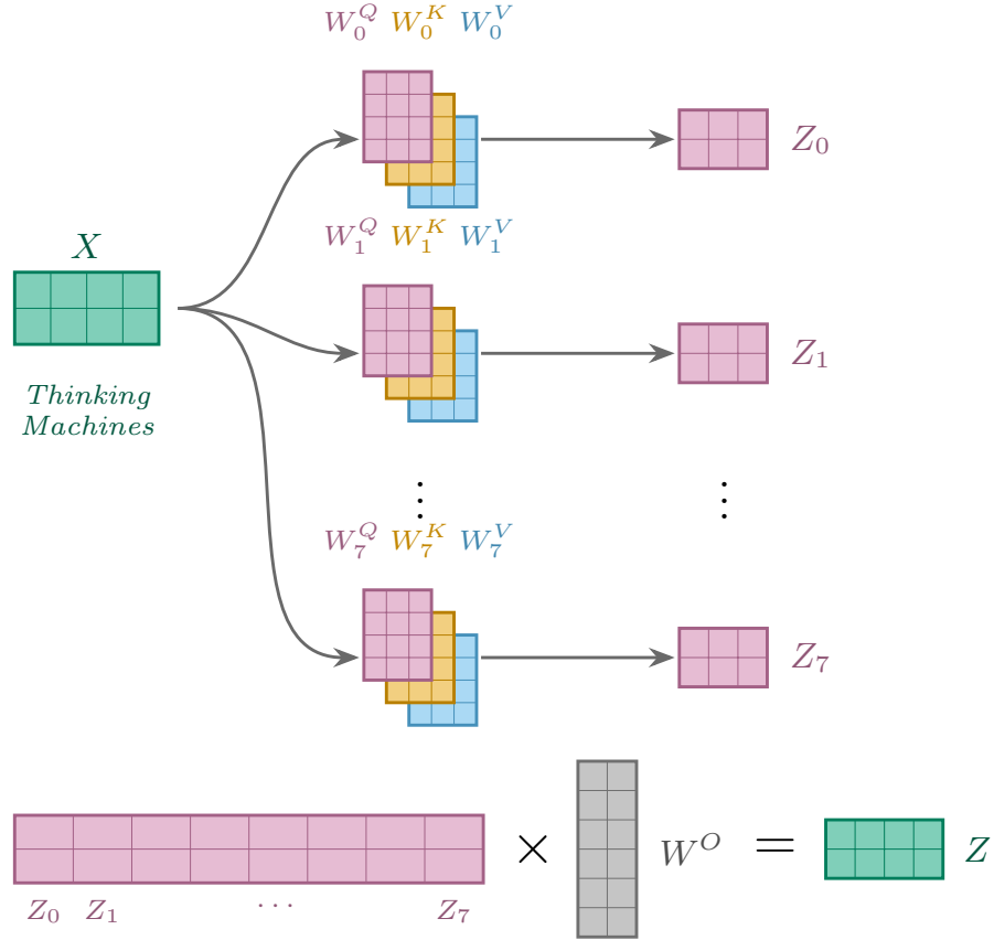
Figure 40: Multi-head attention. The input X is projected by h independent sets of weight matrices W_i^Q, W_i^K, W_i^V , producing one attention output Z_i per head. The heads are concatenated and projected by W^O to obtain the final output Z .
